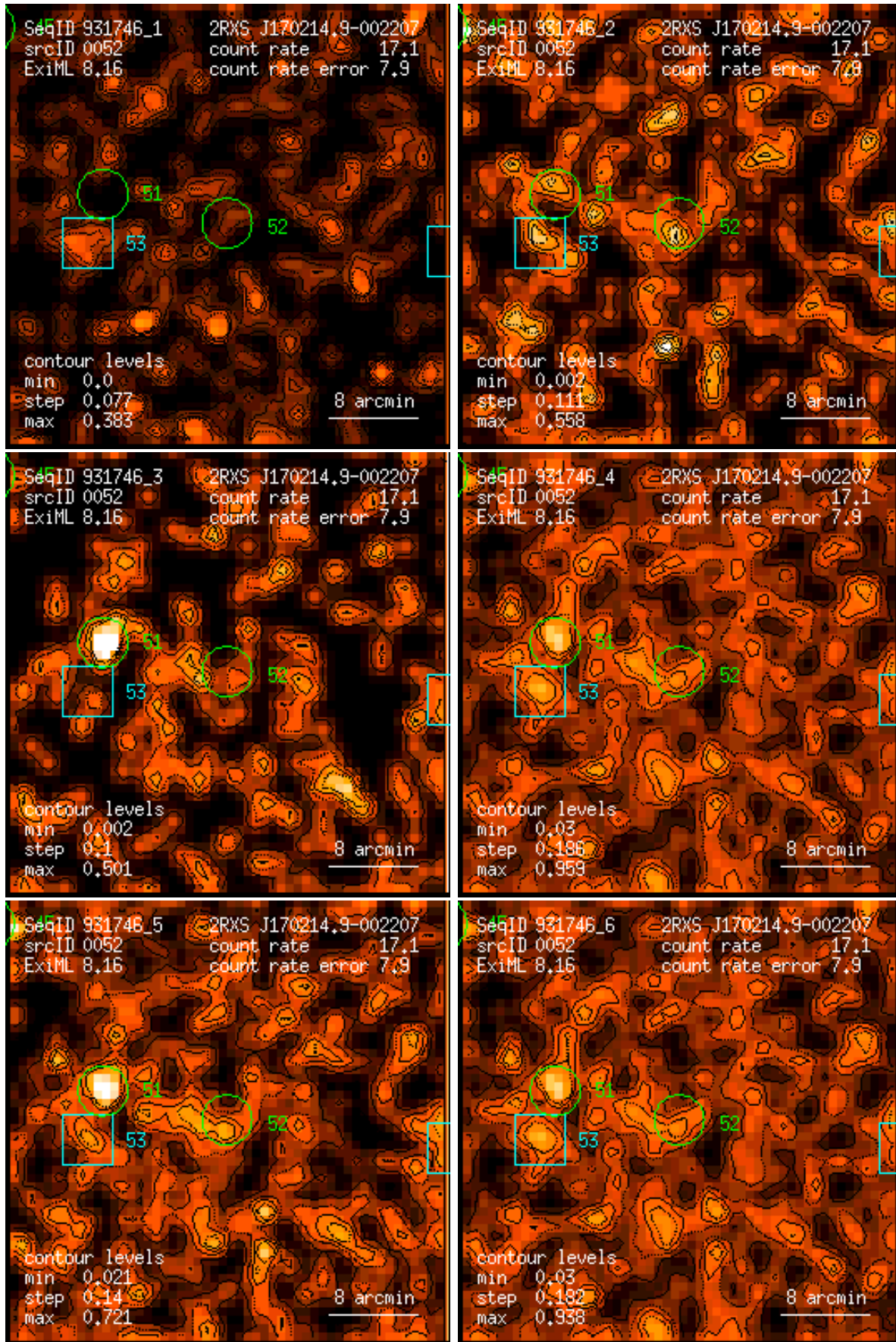
Figure 52: RASS 931746: detection 0052: band rate images, Gaussian filter: (1) PSPC channels 11 – 41, (2) 52 – 90, (3) 91 – 201, (4) 11 – 235, (5) 52 – 201, (6) 11 – 201. Broad band rates in counts/ks. Band rate contour levels in counts/ks/arcmin 2 .
