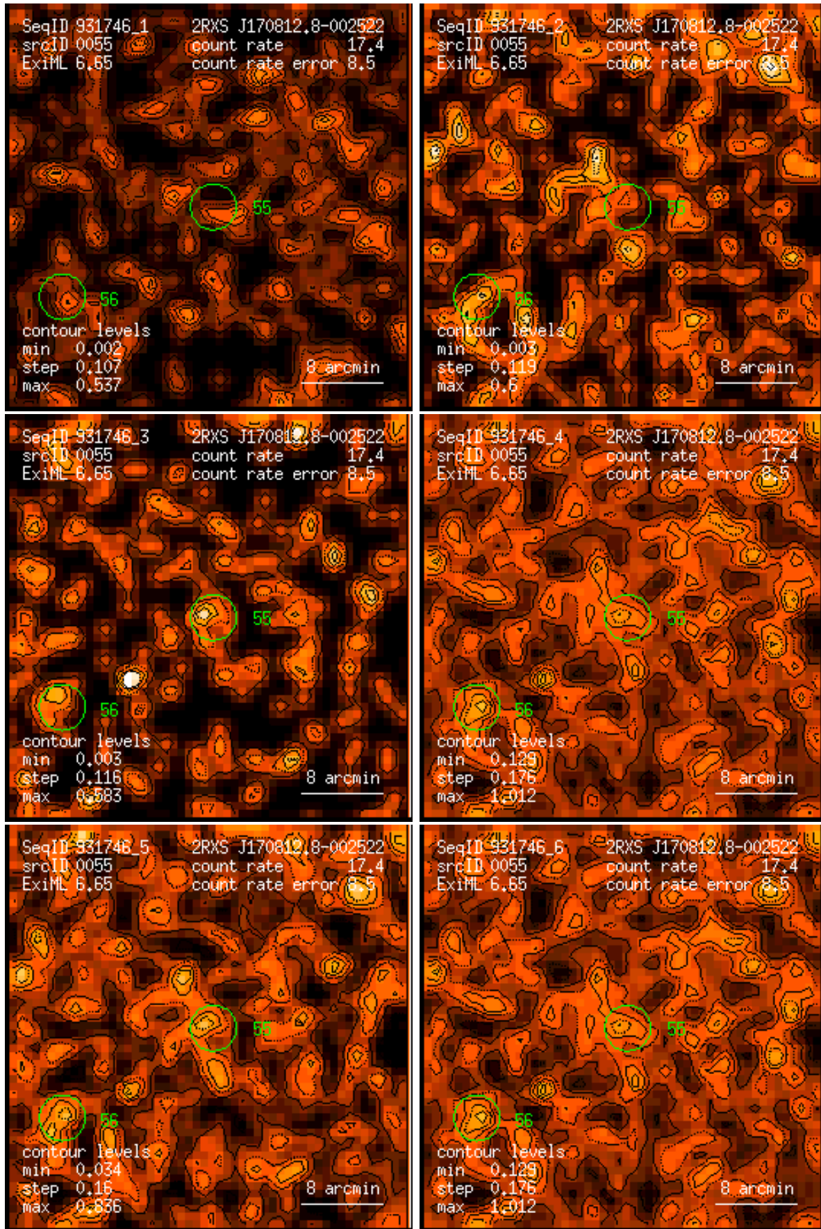
Figure 55: RASS 931746: detection 0055: band rate images, Gaussian filter: (1) PSPC channels 11 – 41, (2) 52 – 90, (3) 91 – 201, (4) 11 – 235, (5) 52 – 201, (6) 11 – 201. Broad band rates in counts/ks. Band rate contour levels in counts/ks/arcmin 2 .
