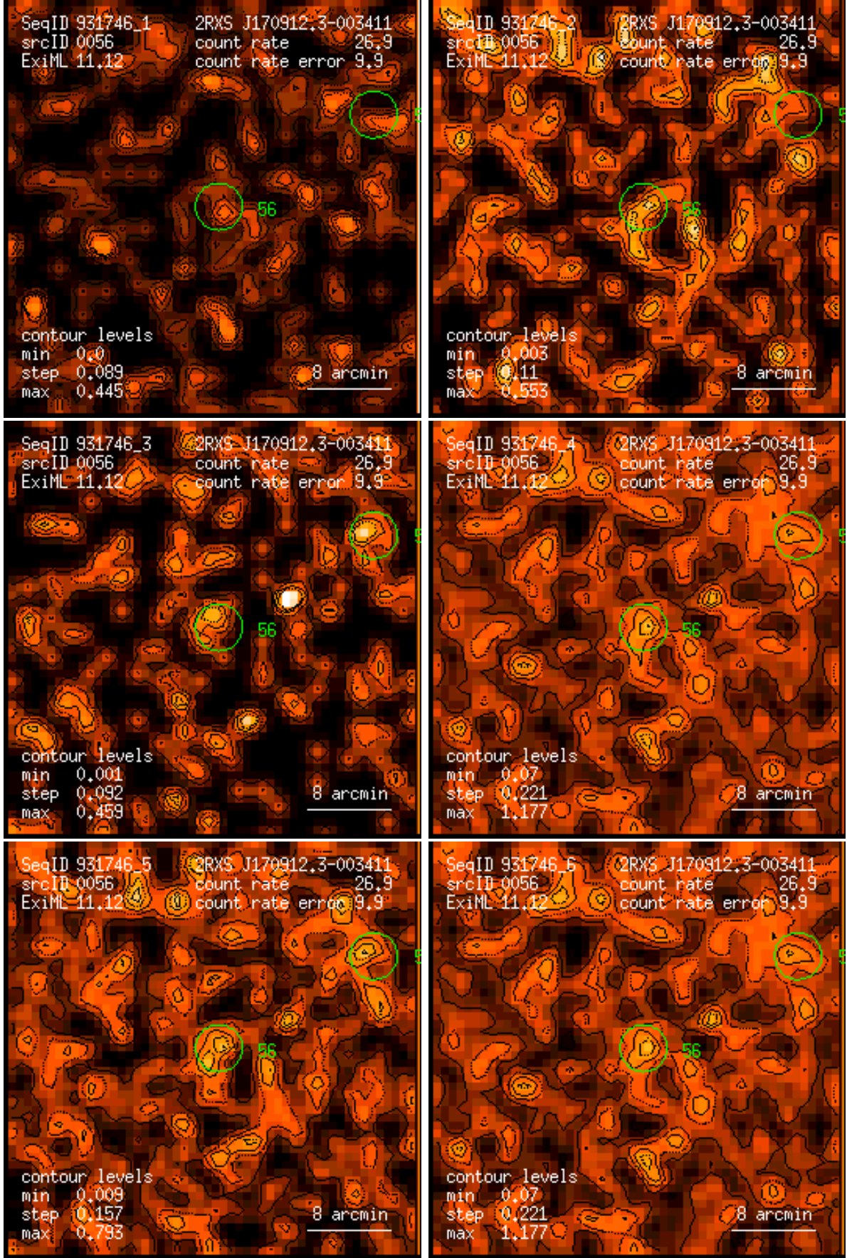
Figure 56: RASS 931746: detection 0056: band rate images, Gaussian filter: (1) PSPC channels 11 – 41, (2) 52 – 90, (3) 91 – 201, (4) 11 – 235, (5) 52 – 201, (6) 11 – 201. Broad band rates in counts/ks. Band rate contour levels in counts/ks/arcmin 2 .
