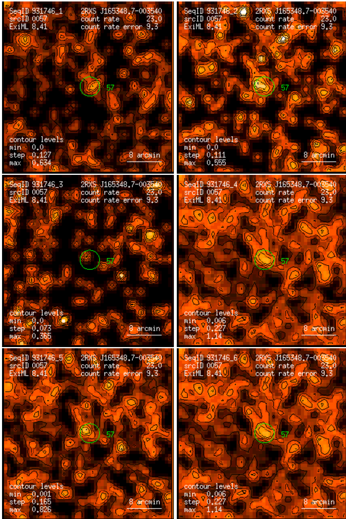
Figure 57: RASS 931746: detection 0057: band rate images, Gaussian filter: (1) PSPC channels 11 – 41, (2) 52 – 90, (3) 91 – 201, (4) 11 – 235, (5) 52 – 201, (6) 11 – 201. Broad band rates in counts/ks. Band rate contour levels in counts/ks/arcmin 2 .
