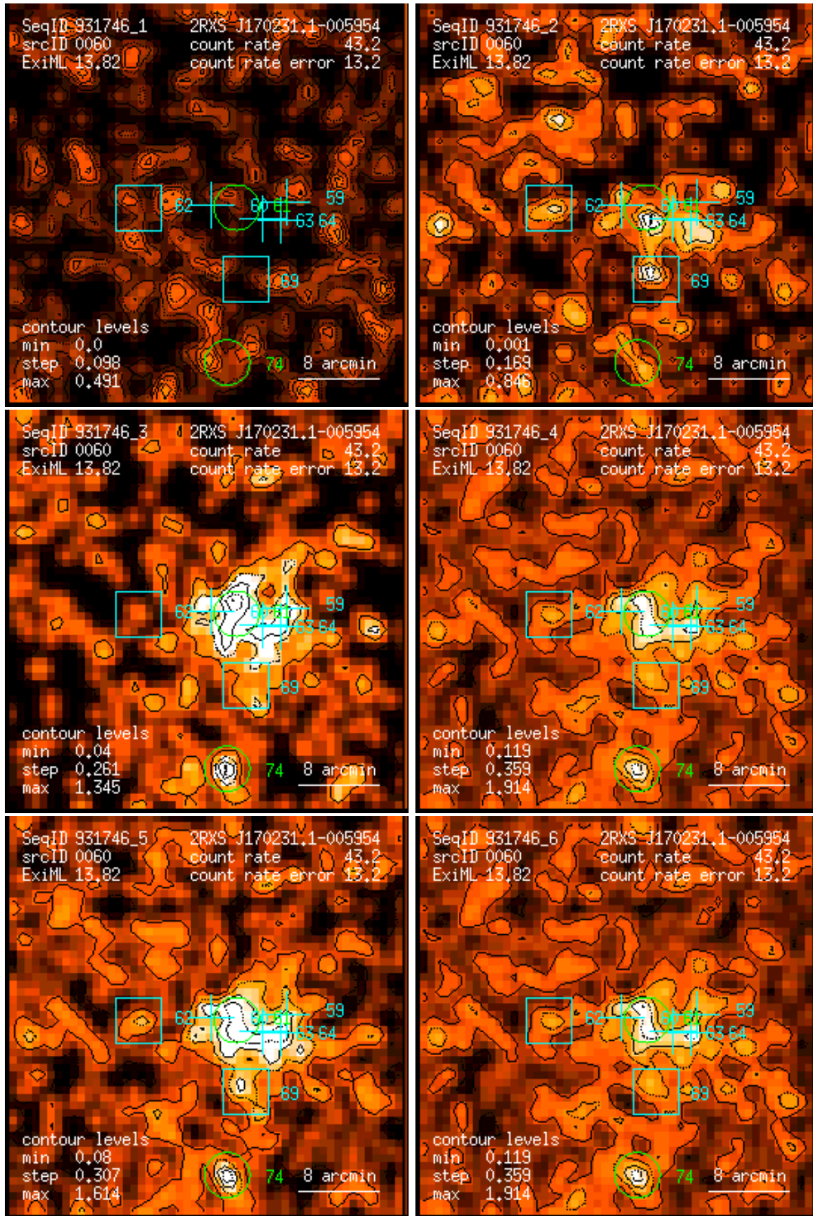
Figure 60: RASS 931746: detection 0060: band rate images, Gaussian filter: (1) PSPC channels 11 – 41, (2) 52 – 90, (3) 91 – 201, (4) 11 – 235, (5) 52 – 201, (6) 11 – 201. Broad band rates in counts/ks. Band rate contour levels in counts/ks/arcmin 2 .
