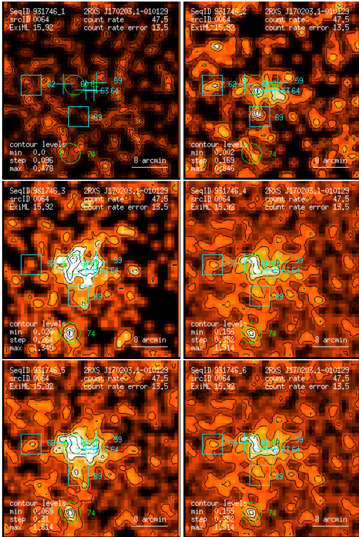
Figure 64: RASS 931746: detection 0064: band rate images, Gaussian filter: (1) PSPC channels 11 – 41, (2) 52 – 90, (3) 91 – 201, (4) 11 – 235, (5) 52 – 201, (6) 11 – 201. Broad band rates in counts/ks. Band rate contour levels in counts/ks/arcmin 2 .
