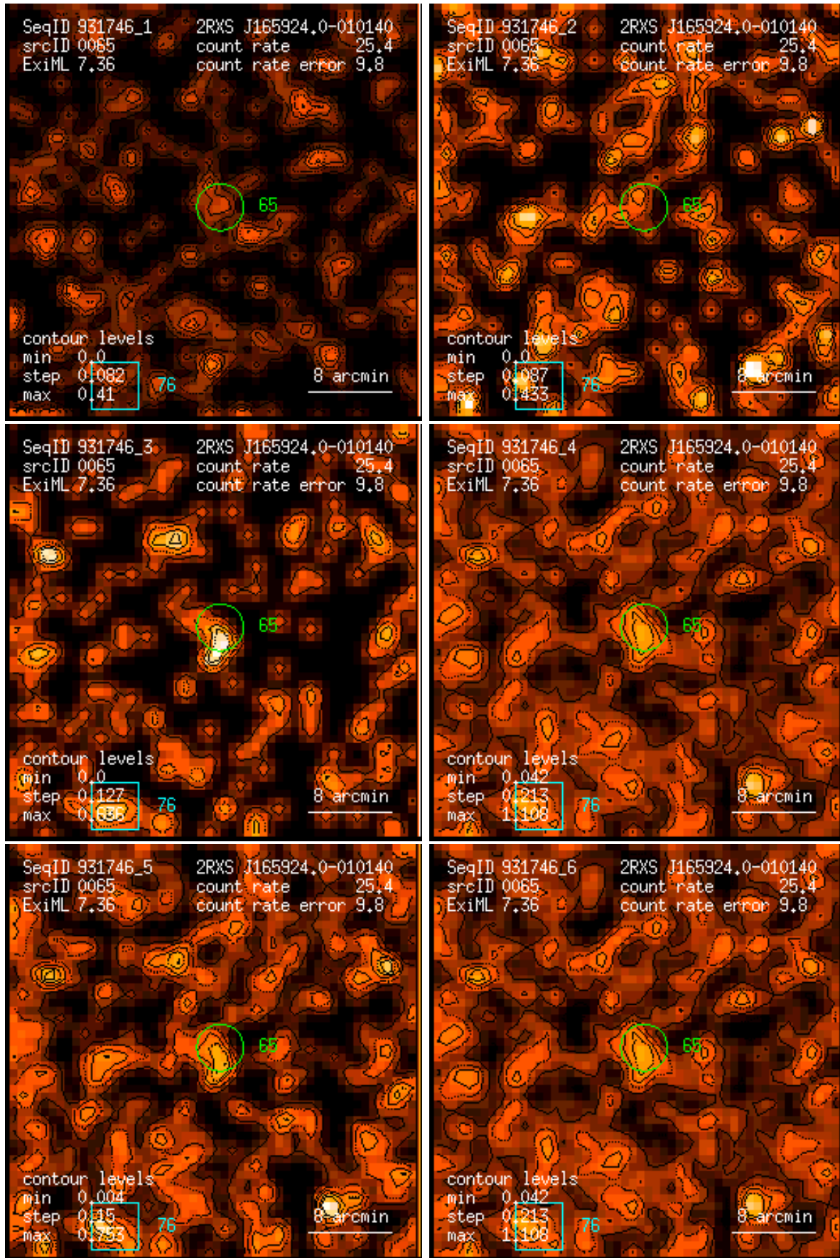
Figure 65: RASS 931746: detection 0065: band rate images, Gaussian filter: (1) PSPC channels 11 – 41, (2) 52 – 90, (3) 91 – 201, (4) 11 – 235, (5) 52 – 201, (6) 11 – 201. Broad band rates in counts/ks. Band rate contour levels in counts/ks/arcmin 2 .
