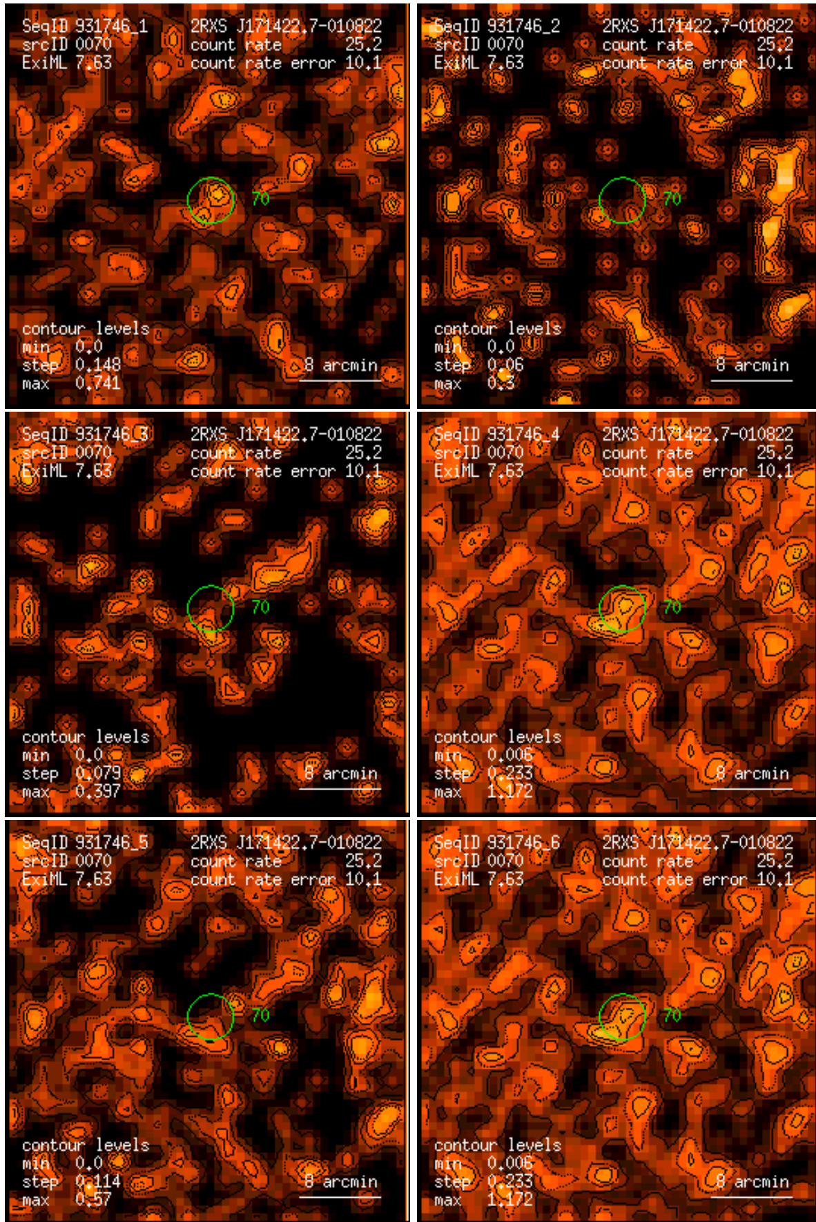
Figure 70: RASS 931746: detection 0070: band rate images, Gaussian filter: (1) PSPC channels 11 – 41, (2) 52 – 90, (3) 91 – 201, (4) 11 – 235, (5) 52 – 201, (6) 11 – 201. Broad band rates in counts/ks. Band rate contour levels in counts/ks/arcmin 2 .
