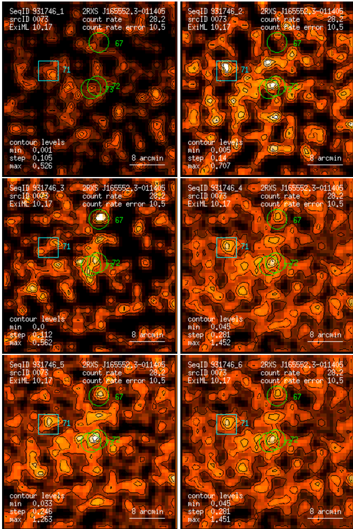
Figure 73: RASS 931746: detection 0073: band rate images, Gaussian filter: (1) PSPC channels 11 – 41, (2) 52 – 90, (3) 91 – 201, (4) 11 – 235, (5) 52 – 201, (6) 11 – 201. Broad band rates in counts/ks. Band rate contour levels in counts/ks/arcmin 2 .
