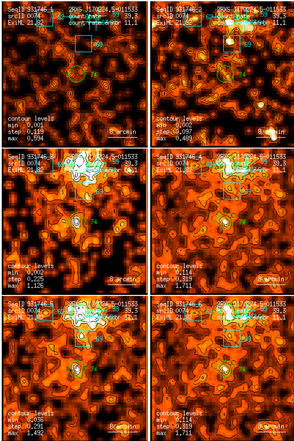
Figure 74: RASS 931746: detection 0074: band rate images, Gaussian filter: (1) PSPC channels 11 – 41, (2) 52 – 90, (3) 91 – 201, (4) 11 – 235, (5) 52 – 201, (6) 11 – 201. Broad band rates in counts/ks. Band rate contour levels in counts/ks/arcmin 2 .
