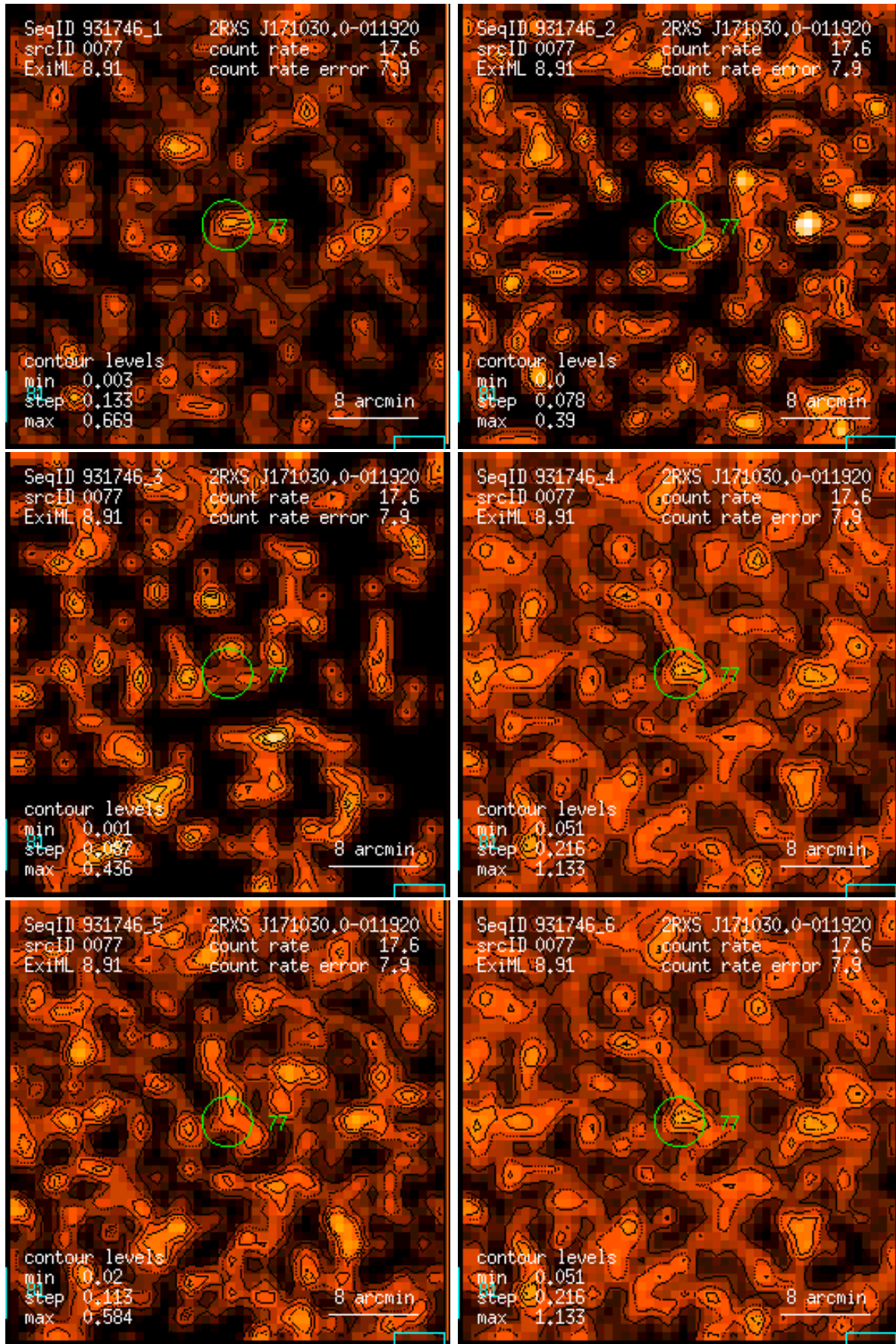
Figure 77: RASS 931746: detection 0077: band rate images, Gaussian filter: (1) PSPC channels 11 – 41, (2) 52 – 90, (3) 91 – 201, (4) 11 – 235, (5) 52 – 201, (6) 11 – 201. Broad band rates in counts/ks. Band rate contour levels in counts/ks/arcmin 2 .
