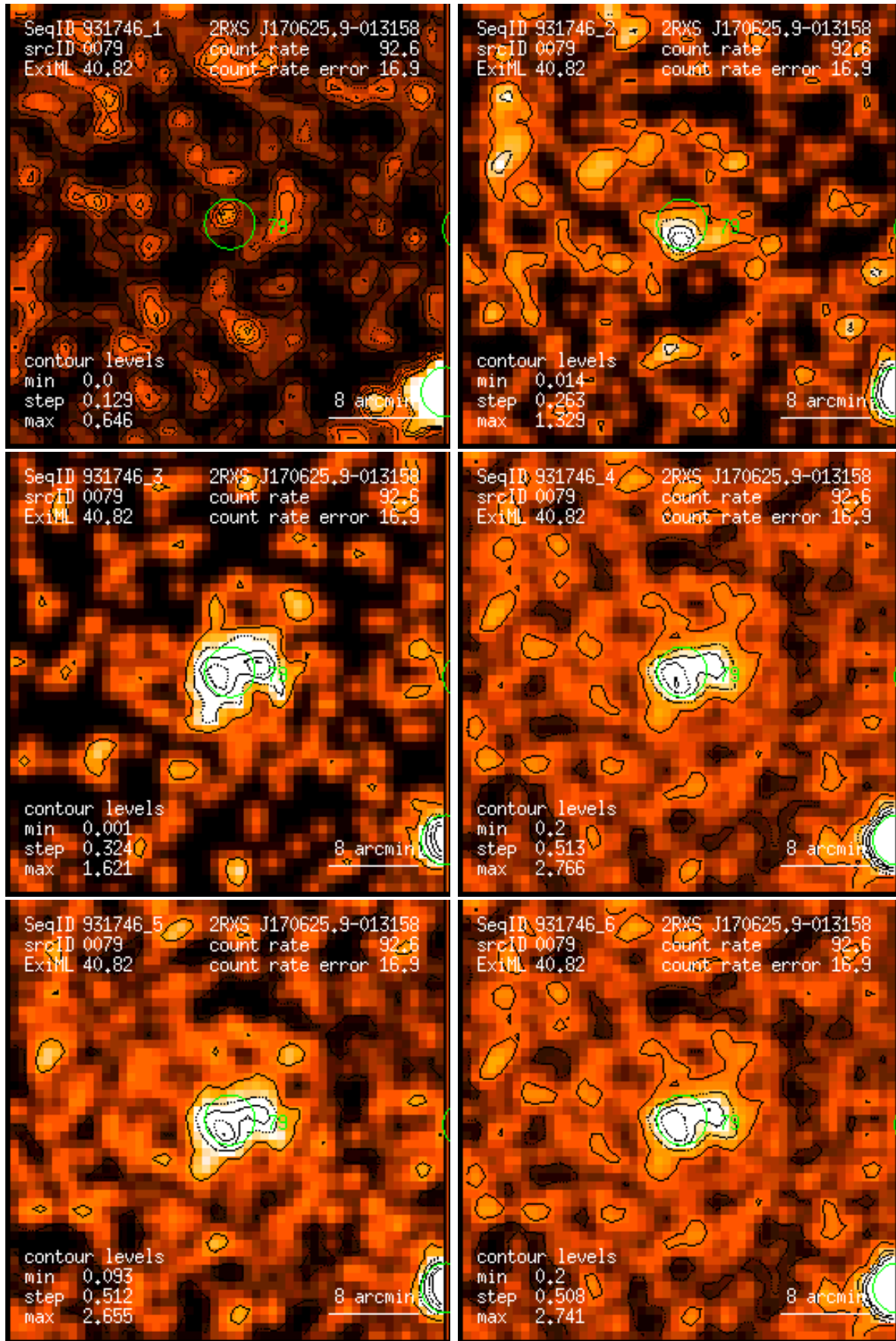
Figure 79: RASS 931746: detection 0079: band rate images, Gaussian filter: (1) PSPC channels 11 – 41, (2) 52 – 90, (3) 91 – 201, (4) 11 – 235, (5) 52 – 201, (6) 11 – 201. Broad band rates in counts/ks. Band rate contour levels in counts/ks/arcmin 2 .
