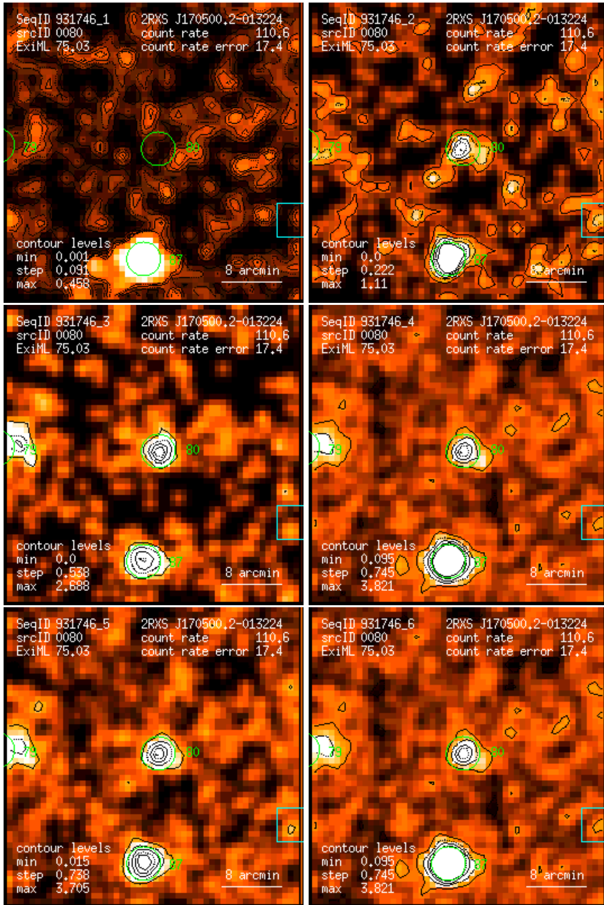
Figure 80: RASS 931746: detection 0080: band rate images, Gaussian filter: (1) PSPC channels 11 – 41, (2) 52 – 90, (3) 91 – 201, (4) 11 – 235, (5) 52 – 201, (6) 11 – 201. Broad band rates in counts/ks. Band rate contour levels in counts/ks/arcmin 2 .
