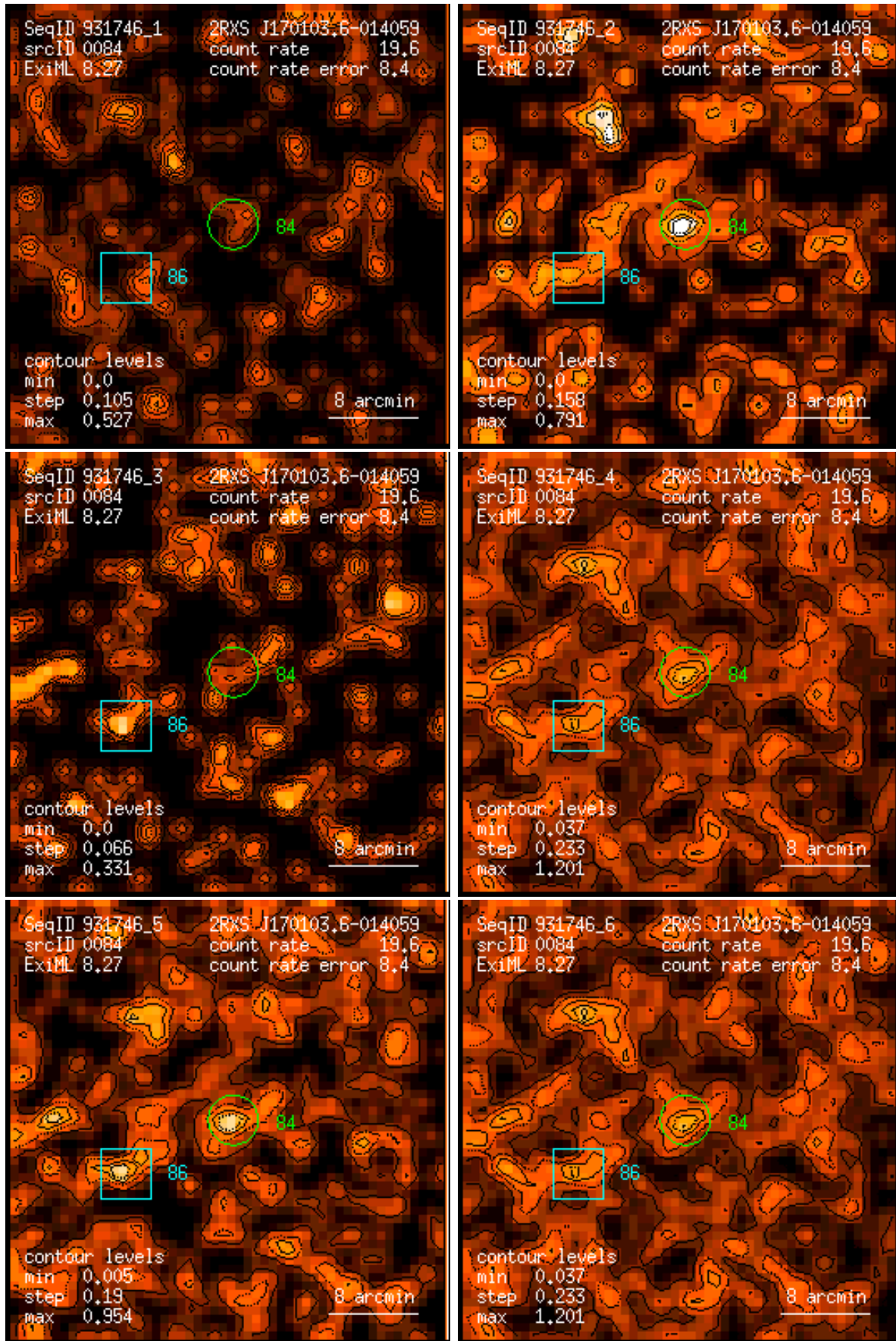
Figure 84: RASS 931746: detection 0084: band rate images, Gaussian filter: (1) PSPC channels 11 – 41, (2) 52 – 90, (3) 91 – 201, (4) 11 – 235, (5) 52 – 201, (6) 11 – 201. Broad band rates in counts/ks. Band rate contour levels in counts/ks/arcmin 2 .
