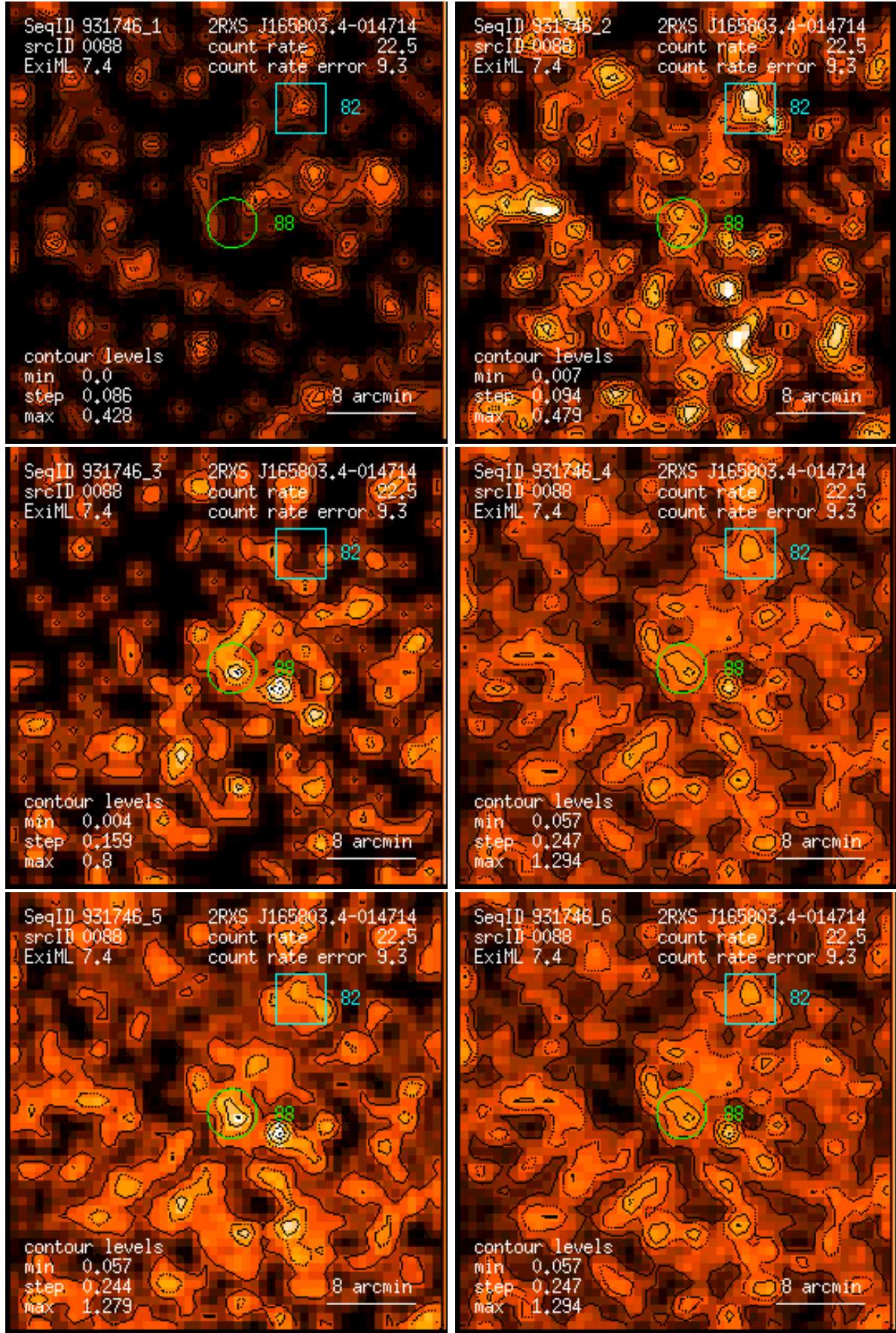
Figure 88: RASS 931746: detection 0088: band rate images, Gaussian filter: (1) PSPC channels 11 – 41, (2) 52 – 90, (3) 91 – 201, (4) 11 – 235, (5) 52 – 201, (6) 11 – 201. Broad band rates in counts/ks. Band rate contour levels in counts/ks/arcmin 2 .
