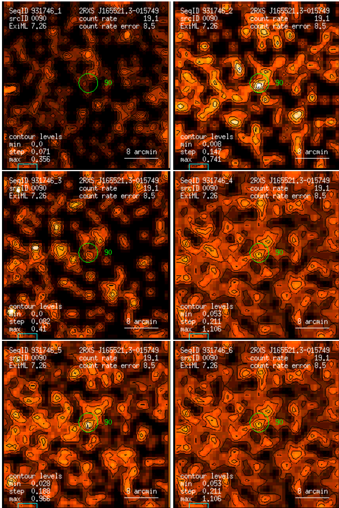
Figure 90: RASS 931746: detection 0090: band rate images, Gaussian filter: (1) PSPC channels 11 – 41, (2) 52 – 90, (3) 91 – 201, (4) 11 – 235, (5) 52 – 201, (6) 11 – 201. Broad band rates in counts/ks. Band rate contour levels in counts/ks/arcmin 2 .
