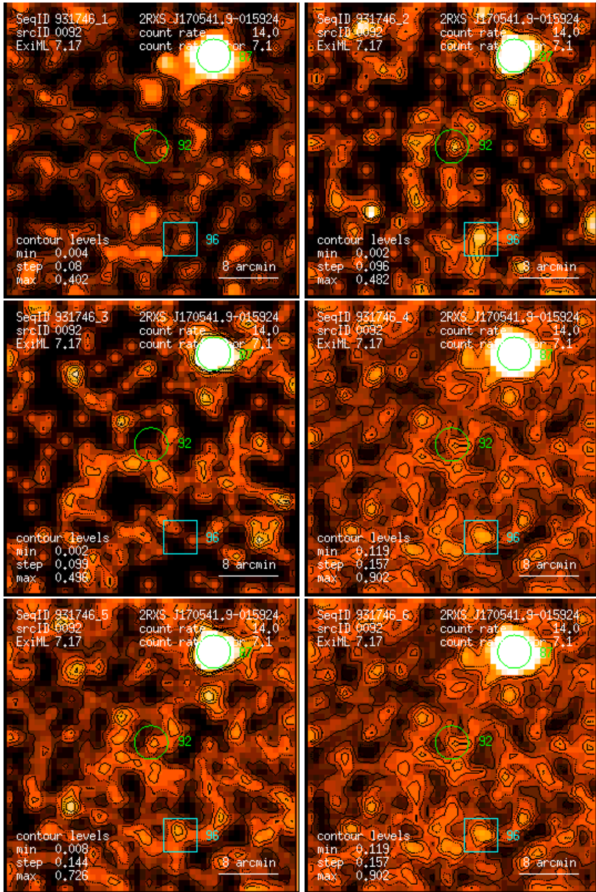
Figure 92: RASS 931746: detection 0092: band rate images, Gaussian filter: (1) PSPC channels 11 – 41, (2) 52 – 90, (3) 91 – 201, (4) 11 – 235, (5) 52 – 201, (6) 11 – 201. Broad band rates in counts/ks. Band rate contour levels in counts/ks/arcmin 2 .
