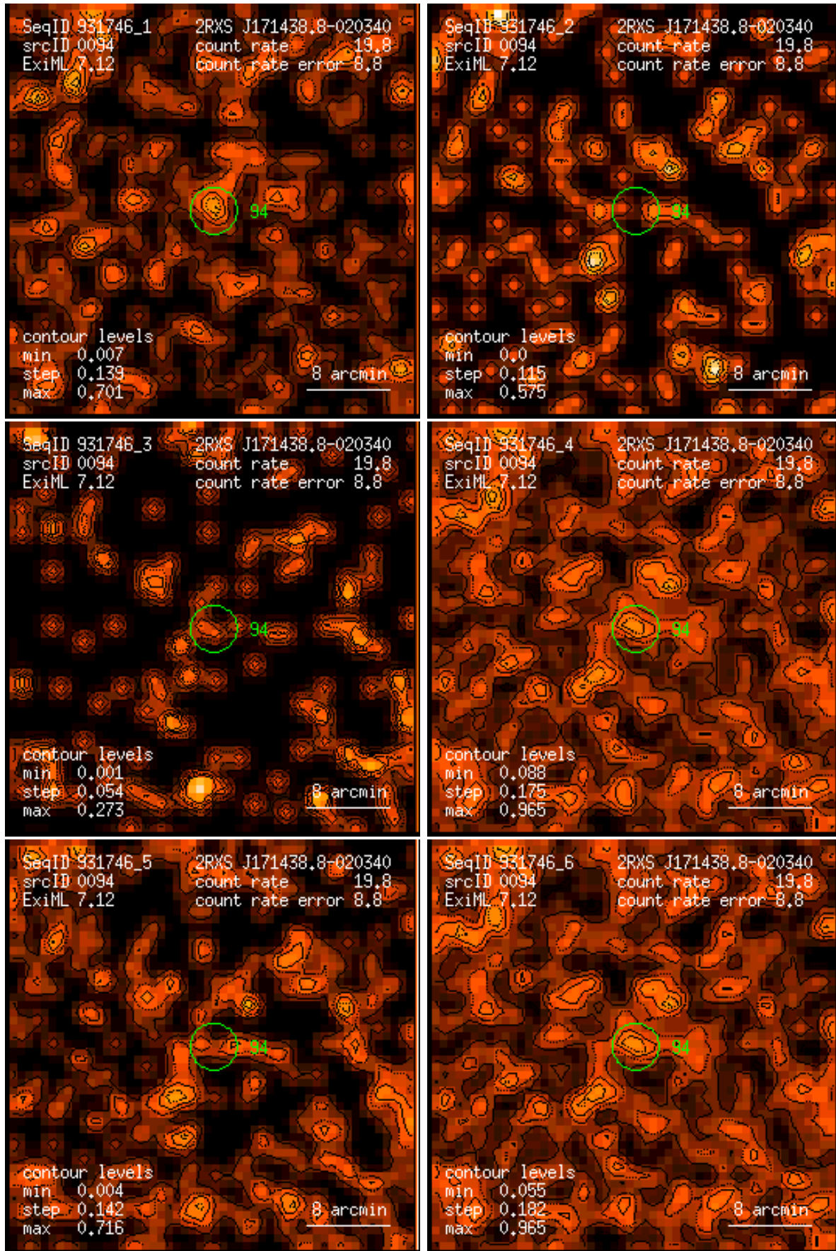
Figure 94: RASS 931746: detection 0094: band rate images, Gaussian filter: (1) PSPC channels 11 – 41, (2) 52 – 90, (3) 91 – 201, (4) 11 – 235, (5) 52 – 201, (6) 11 – 201. Broad band rates in counts/ks. Band rate contour levels in counts/ks/arcmin 2 .
