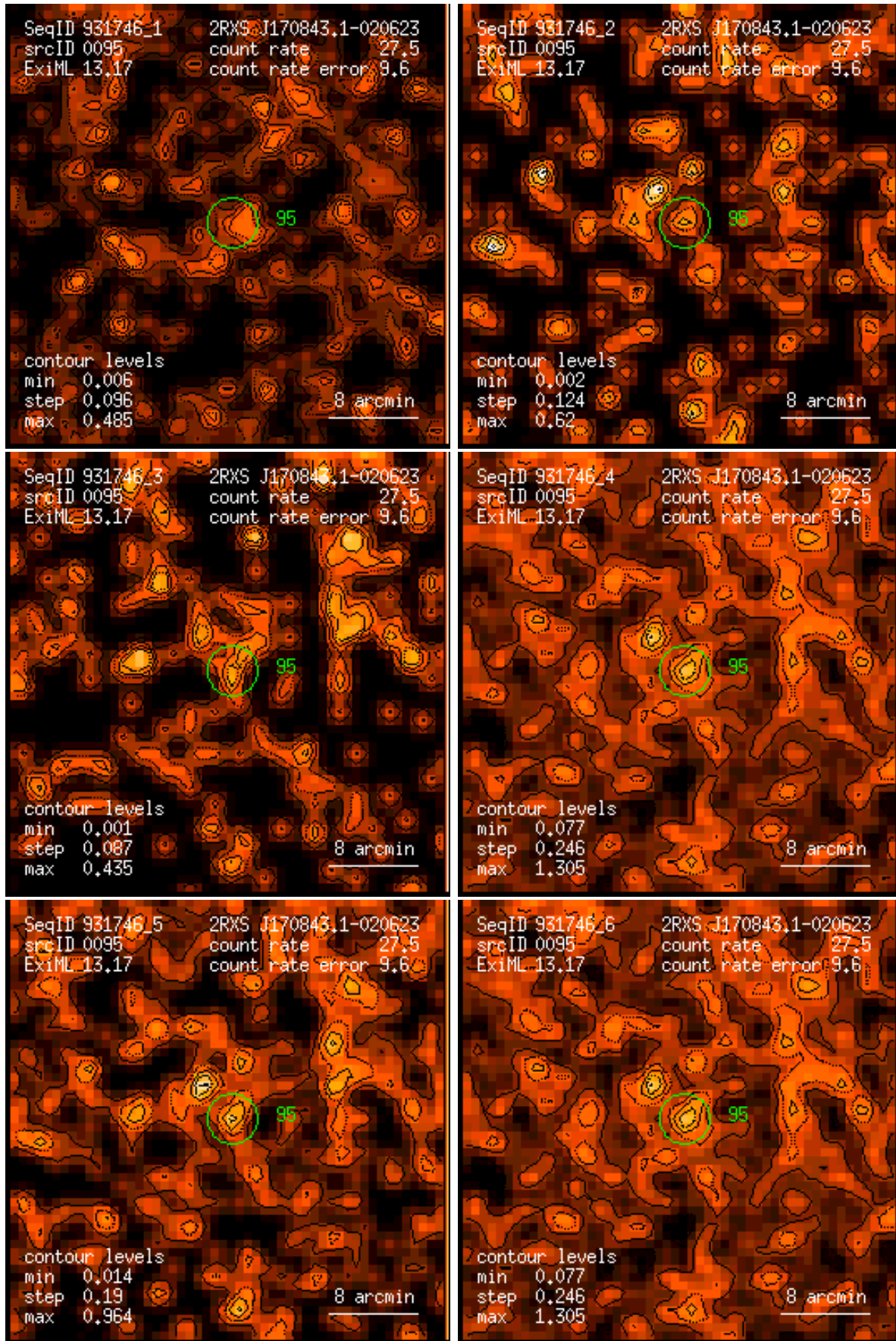
Figure 95: RASS 931746: detection 0095: band rate images, Gaussian filter: (1) PSPC channels 11 – 41, (2) 52 – 90, (3) 91 – 201, (4) 11 – 235, (5) 52 – 201, (6) 11 – 201. Broad band rates in counts/ks. Band rate contour levels in counts/ks/arcmin 2 .
