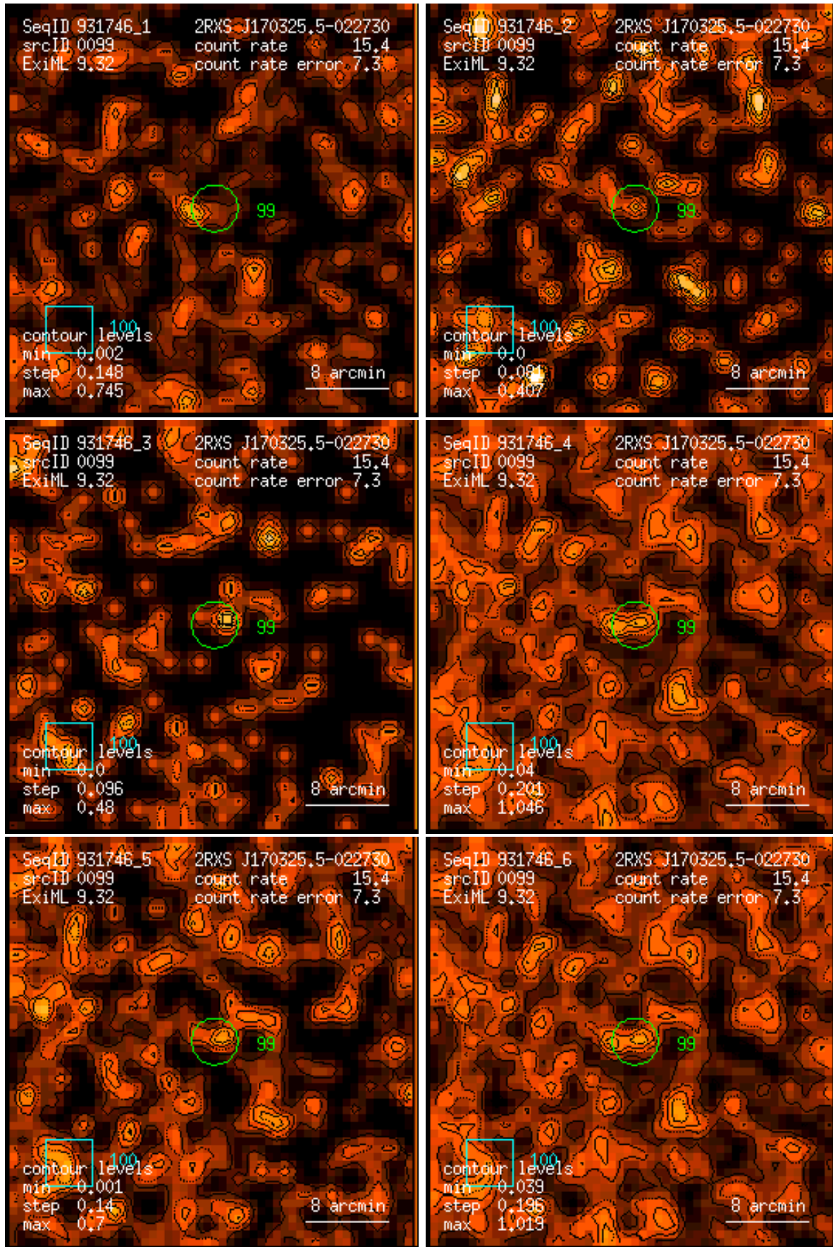
Figure 99: RASS 931746: detection 0099: band rate images, Gaussian filter: (1) PSPC channels 11 – 41, (2) 52 – 90, (3) 91 – 201, (4) 11 – 235, (5) 52 – 201, (6) 11 – 201. Broad band rates in counts/ks. Band rate contour levels in counts/ks/arcmin 2 .
