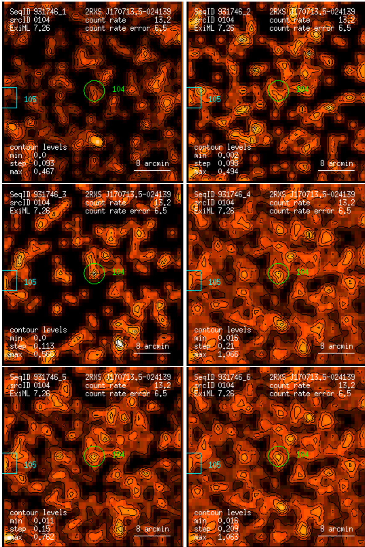
Figure 104: RASS 931746: detection 0104: band rate images, Gaussian filter: (1) PSPC channels 11 – 41, (2) 52 – 90, (3) 91 – 201, (4) 11 – 235, (5) 52 – 201, (6) 11 – 201. Broad band rates in counts/ks. Band rate contour levels in counts/ks/arcmin 2 .
