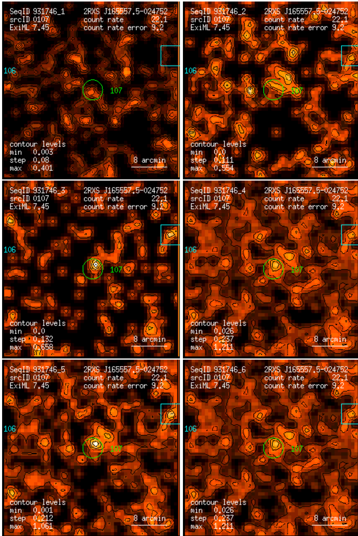
Figure 107: RASS 931746: detection 0107: band rate images, Gaussian filter: (1) PSPC channels 11 – 41, (2) 52 – 90, (3) 91 – 201, (4) 11 – 235, (5) 52 – 201, (6) 11 – 201. Broad band rates in counts/ks. Band rate contour levels in counts/ks/arcmin 2 .
