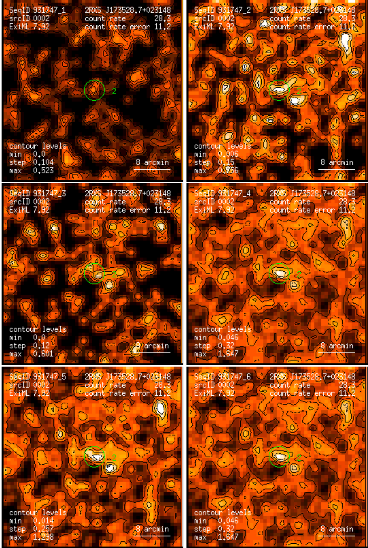
Figure 2: RASS 931747: detection 0002: band rate images, Gaussian filter: (1) PSPC channels 11 – 41, (2) 52 – 90, (3) 91 – 201, (4) 11 – 235, (5) 52 – 201, (6) 11 – 201. Broad band rates in counts/ks. Band rate contour levels in counts/ks/arcmin 2 .
