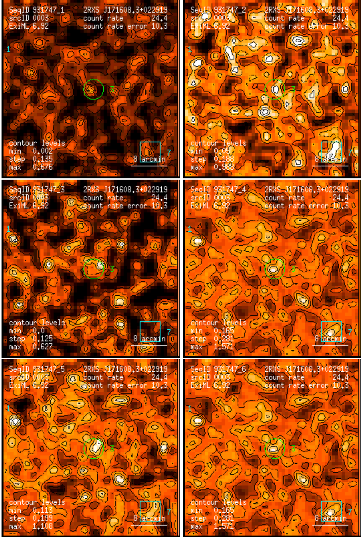
Figure 3: RASS 931747: detection 0003: band rate images, Gaussian filter: (1) PSPC channels 11 – 41, (2) 52 – 90, (3) 91 – 201, (4) 11 – 235, (5) 52 – 201, (6) 11 – 201. Broad band rates in counts/ks. Band rate contour levels in counts/ks/arcmin 2 .
