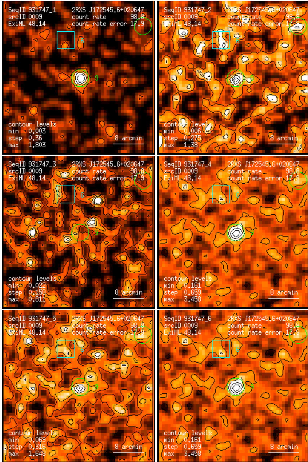
Figure 9: RASS 931747: detection 0009: band rate images, Gaussian filter: (1) PSPC channels 11 – 41, (2) 52 – 90, (3) 91 – 201, (4) 11 – 235, (5) 52 – 201, (6) 11 – 201. Broad band rates in counts/ks. Band rate contour levels in counts/ks/arcmin 2 .
