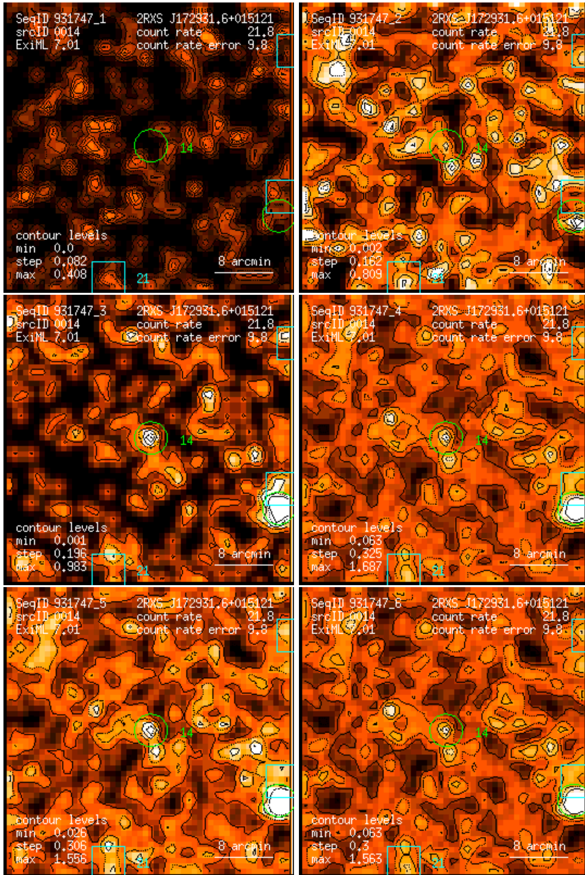
Figure 14: RASS 931747: detection 0014: band rate images, Gaussian filter: (1) PSPC channels 11 – 41, (2) 52 – 90, (3) 91 – 201, (4) 11 – 235, (5) 52 – 201, (6) 11 – 201. Broad band rates in counts/ks. Band rate contour levels in counts/ks/arcmin 2 .
