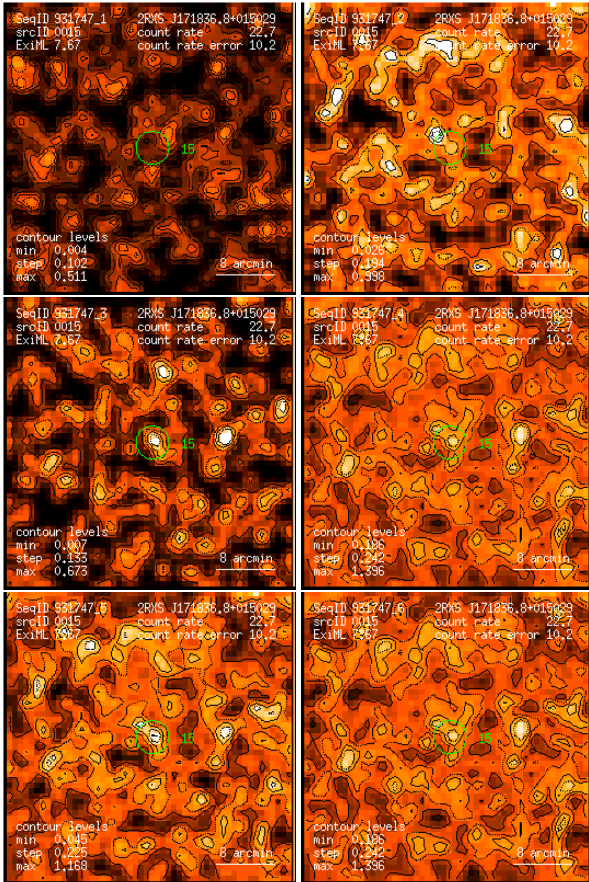
Figure 15: RASS 931747: detection 0015: band rate images, Gaussian filter: (1) PSPC channels 11 – 41, (2) 52 – 90, (3) 91 – 201, (4) 11 – 235, (5) 52 – 201, (6) 11 – 201. Broad band rates in counts/ks. Band rate contour levels in counts/ks/arcmin 2 .
