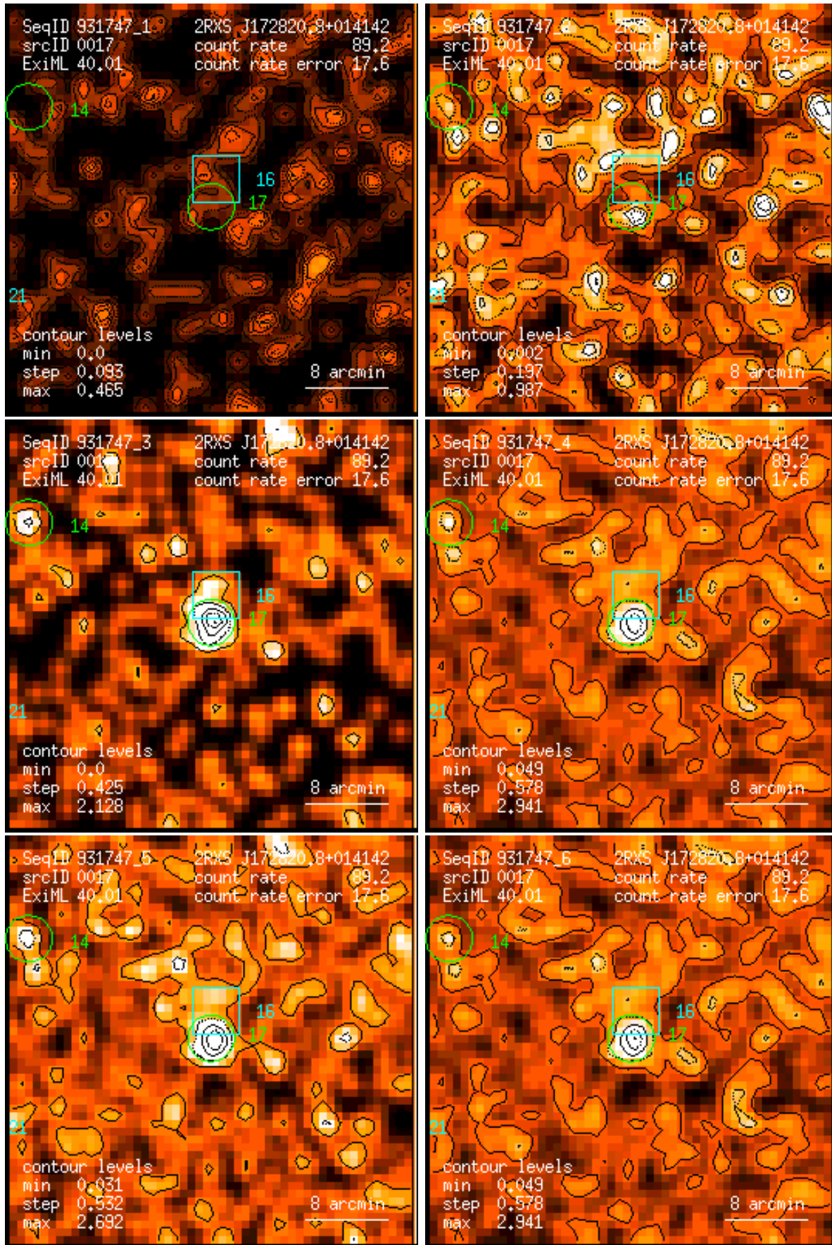
Figure 17: RASS 931747: detection 0017: band rate images, Gaussian filter: (1) PSPC channels 11 – 41, (2) 52 – 90, (3) 91 – 201, (4) 11 – 235, (5) 52 – 201, (6) 11 – 201. Broad band rates in counts/ks. Band rate contour levels in counts/ks/arcmin 2 .
