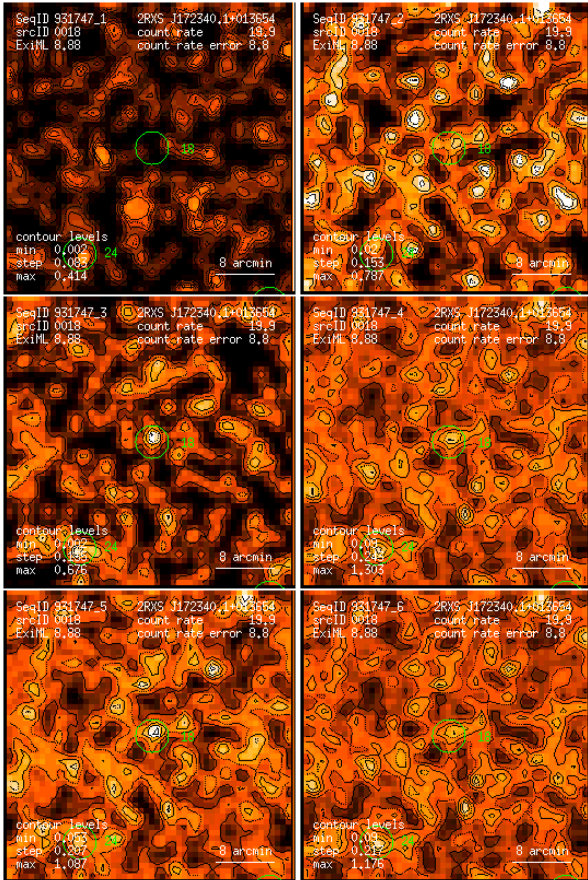
Figure 18: RASS 931747: detection 0018: band rate images, Gaussian filter: (1) PSPC channels 11 – 41, (2) 52 – 90, (3) 91 – 201, (4) 11 – 235, (5) 52 – 201, (6) 11 – 201. Broad band rates in counts/ks. Band rate contour levels in counts/ks/arcmin 2 .
