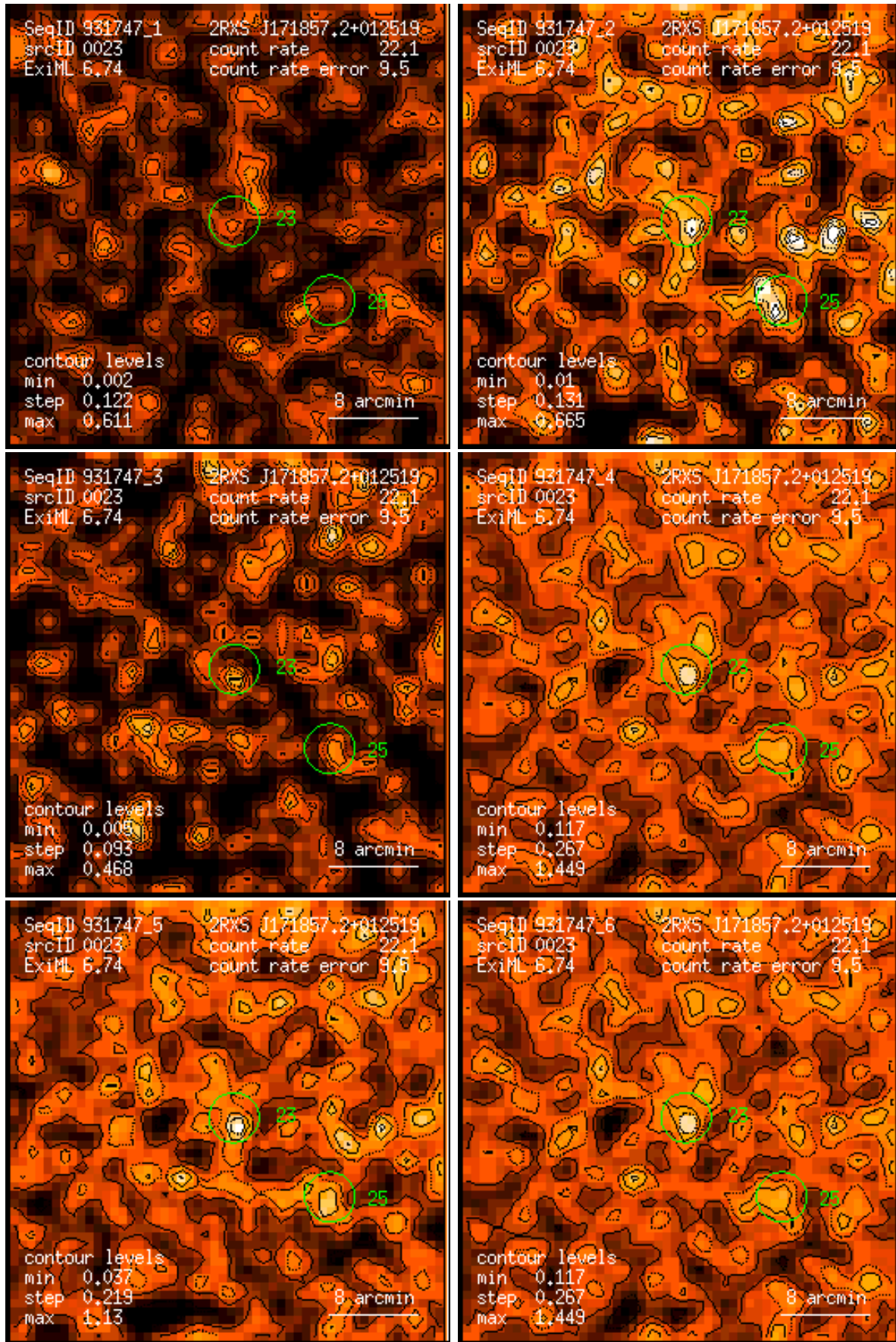
Figure 23: RASS 931747: detection 0023: band rate images, Gaussian filter: (1) PSPC channels 11 – 41, (2) 52 – 90, (3) 91 – 201, (4) 11 – 235, (5) 52 – 201, (6) 11 – 201. Broad band rates in counts/ks. Band rate contour levels in counts/ks/arcmin 2 .
