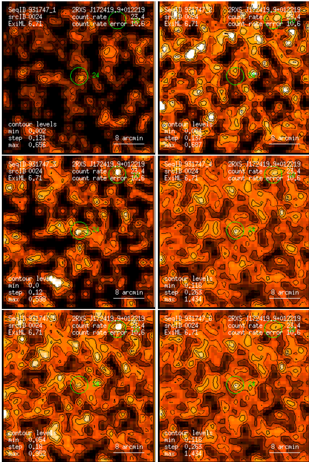
Figure 24: RASS 931747: detection 0024: band rate images, Gaussian filter: (1) PSPC channels 11 – 41, (2) 52 – 90, (3) 91 – 201, (4) 11 – 235, (5) 52 – 201, (6) 11 – 201. Broad band rates in counts/ks. Band rate contour levels in counts/ks/arcmin 2 .
