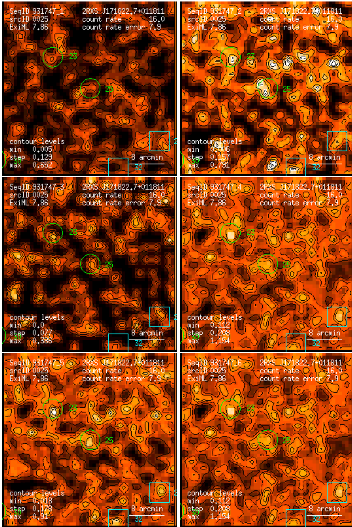
Figure 25: RASS 931747: detection 0025: band rate images, Gaussian filter: (1) PSPC channels 11 – 41, (2) 52 – 90, (3) 91 – 201, (4) 11 – 235, (5) 52 – 201, (6) 11 – 201. Broad band rates in counts/ks. Band rate contour levels in counts/ks/arcmin 2 .
