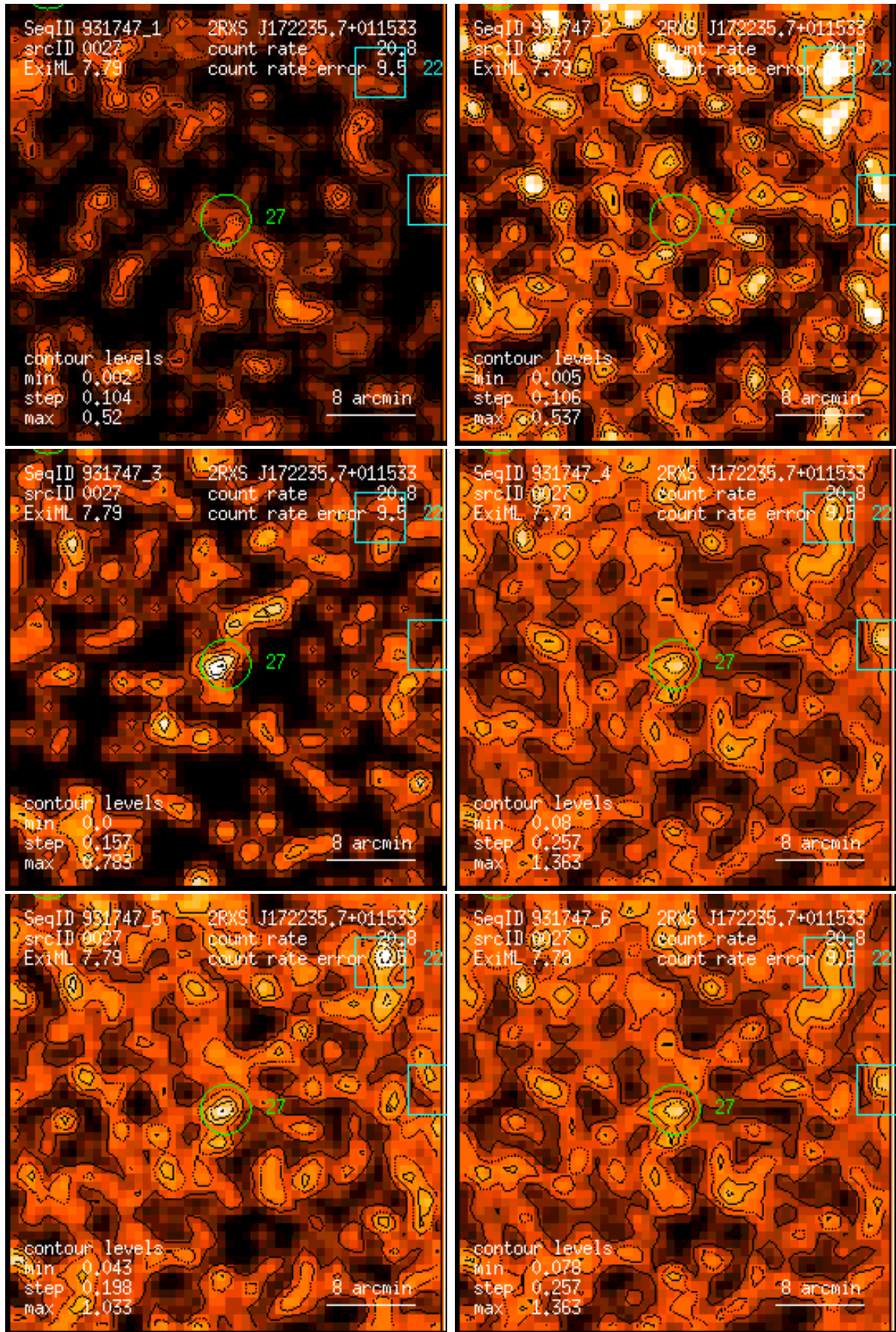
Figure 27: RASS 931747: detection 0027: band rate images, Gaussian filter: (1) PSPC channels 11 – 41, (2) 52 – 90, (3) 91 – 201, (4) 11 – 235, (5) 52 – 201, (6) 11 – 201. Broad band rates in counts/ks. Band rate contour levels in counts/ks/arcmin 2 .
