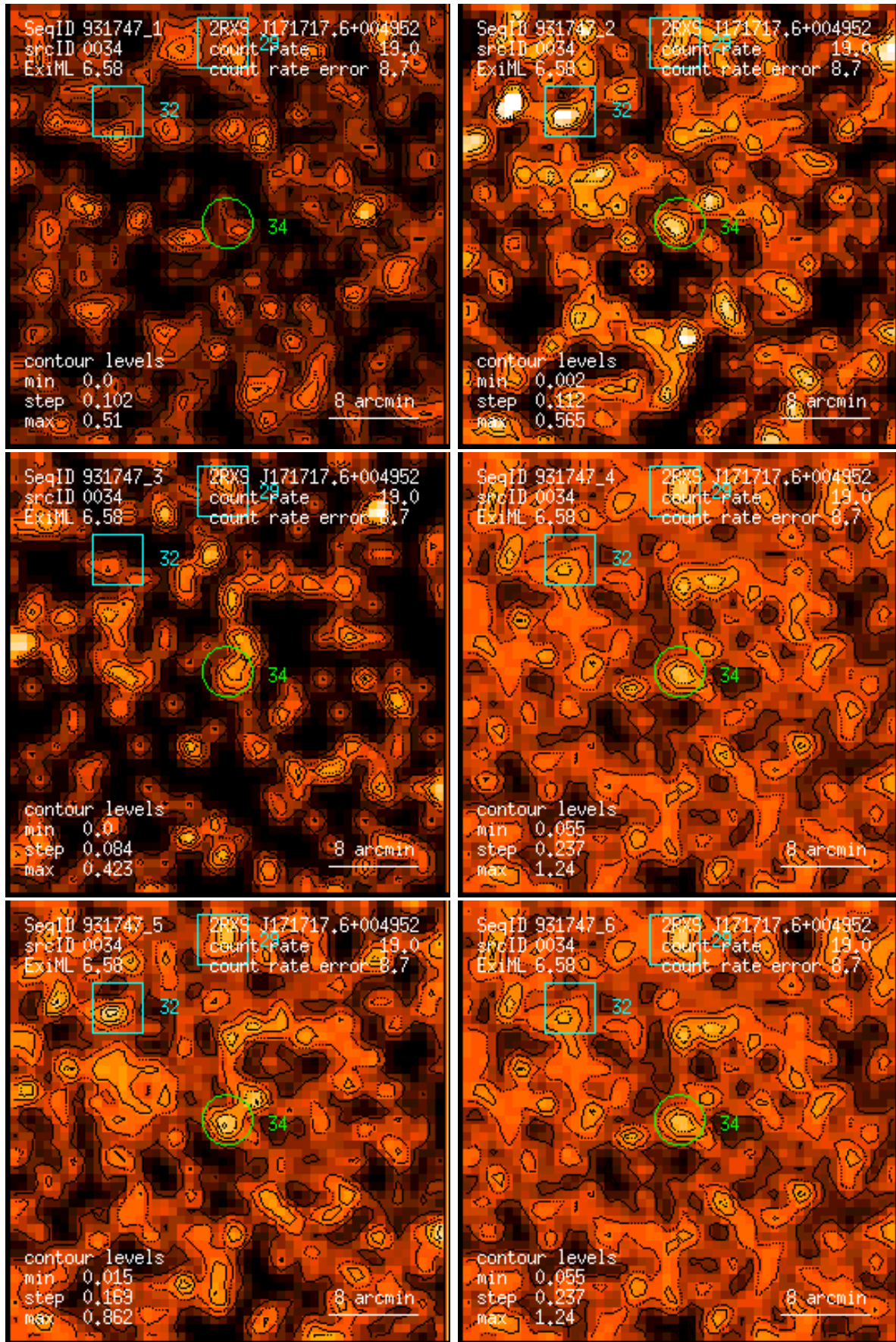
Figure 34: RASS 931747: detection 0034: band rate images, Gaussian filter: (1) PSPC channels 11 – 41, (2) 52 – 90, (3) 91 – 201, (4) 11 – 235, (5) 52 – 201, (6) 11 – 201. Broad band rates in counts/ks. Band rate contour levels in counts/ks/arcmin 2 .
