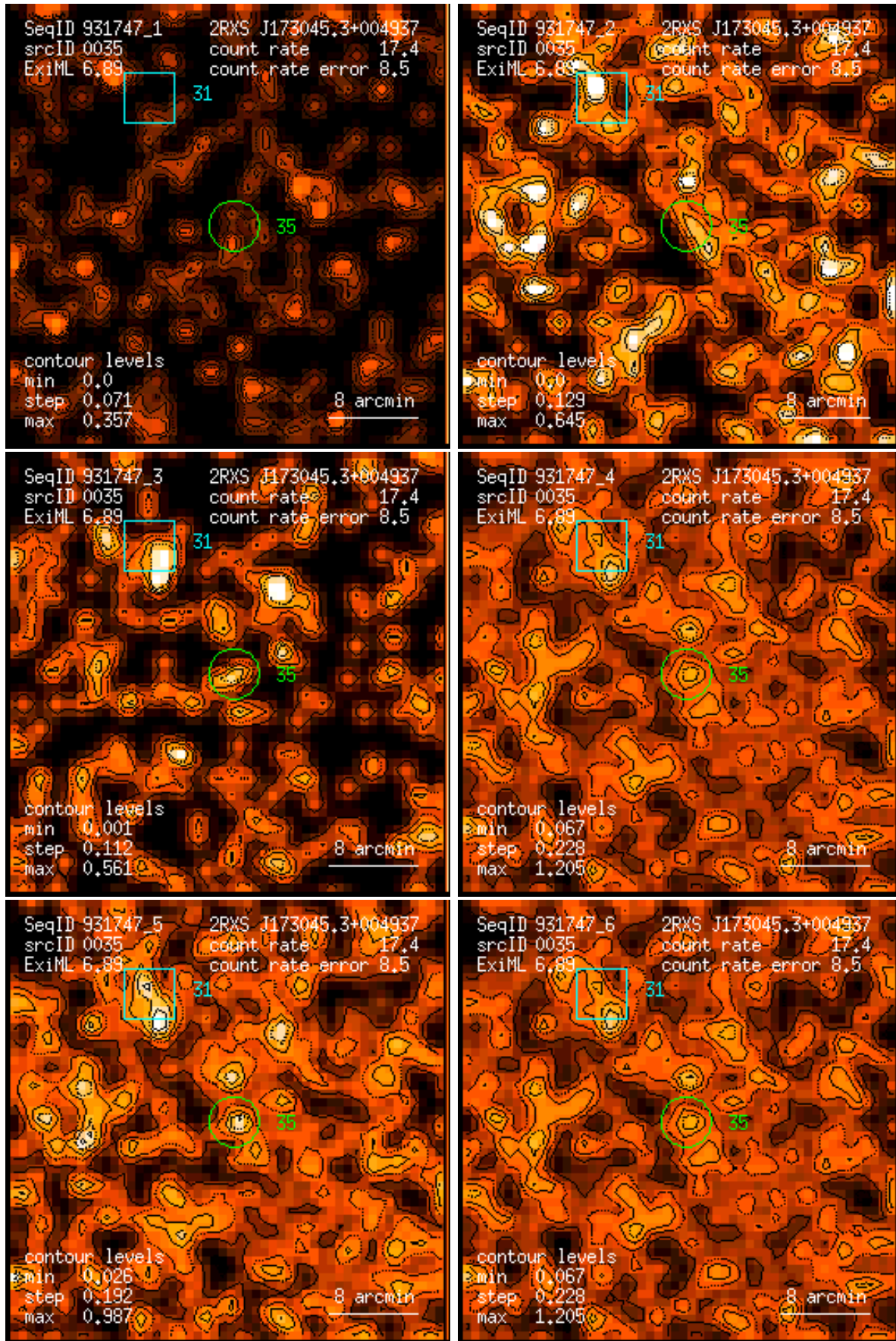
Figure 35: RASS 931747: detection 0035: band rate images, Gaussian filter: (1) PSPC channels 11 – 41, (2) 52 – 90, (3) 91 – 201, (4) 11 – 235, (5) 52 – 201, (6) 11 – 201. Broad band rates in counts/ks. Band rate contour levels in counts/ks/arcmin 2 .
