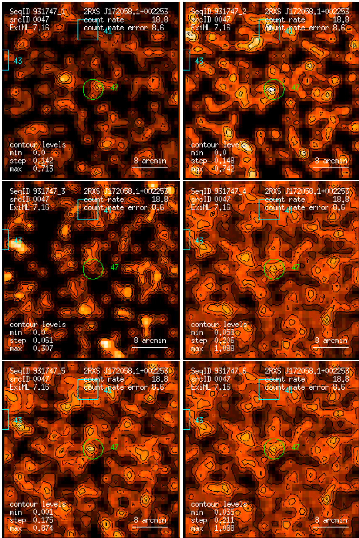
Figure 47: RASS 931747: detection 0047: band rate images, Gaussian filter: (1) PSPC channels 11 – 41, (2) 52 – 90, (3) 91 – 201, (4) 11 – 235, (5) 52 – 201, (6) 11 – 201. Broad band rates in counts/ks. Band rate contour levels in counts/ks/arcmin 2 .
