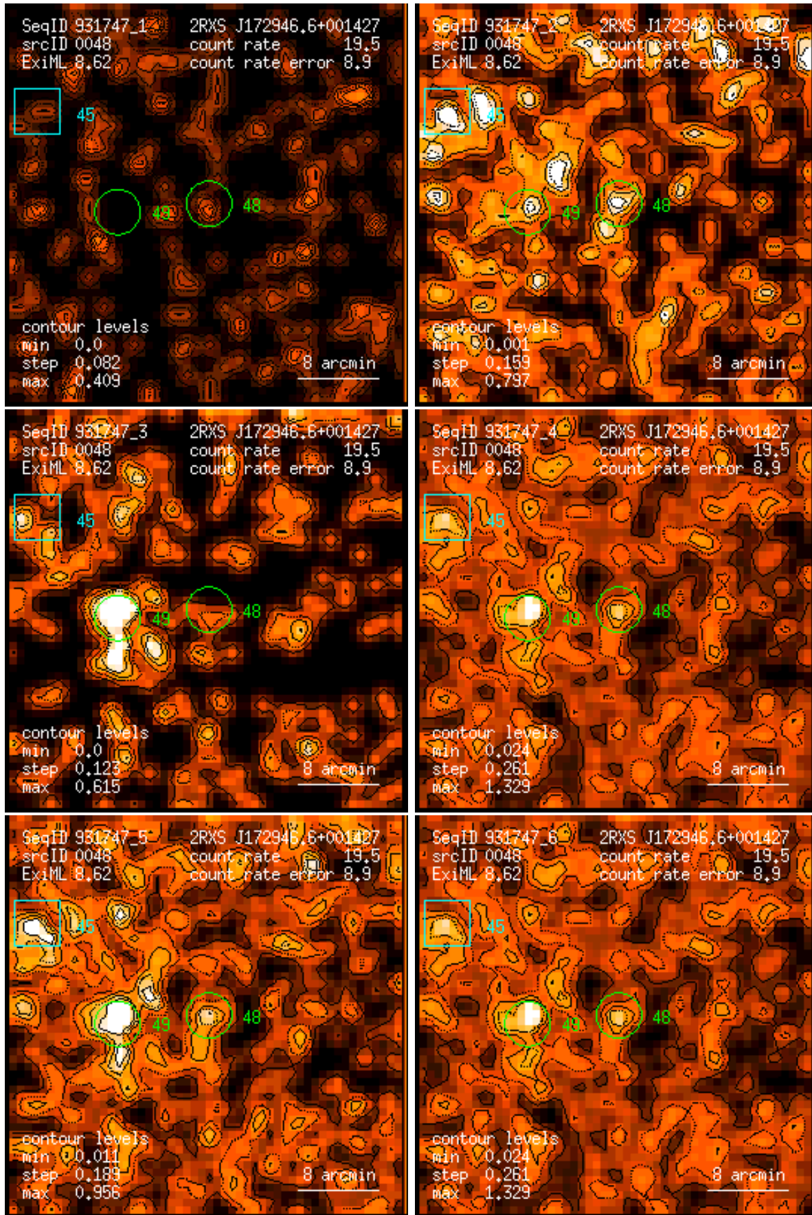
Figure 48: RASS 931747: detection 0048: band rate images, Gaussian filter: (1) PSPC channels 11 – 41, (2) 52 – 90, (3) 91 – 201, (4) 11 – 235, (5) 52 – 201, (6) 11 – 201. Broad band rates in counts/ks. Band rate contour levels in counts/ks/arcmin 2 .
