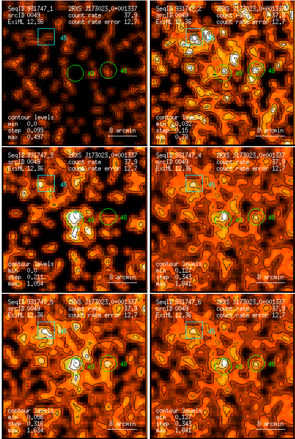
Figure 49: RASS 931747: detection 0049: band rate images, Gaussian filter: (1) PSPC channels 11 – 41, (2) 52 – 90, (3) 91 – 201, (4) 11 – 235, (5) 52 – 201, (6) 11 – 201. Broad band rates in counts/ks. Band rate contour levels in counts/ks/arcmin 2 .
