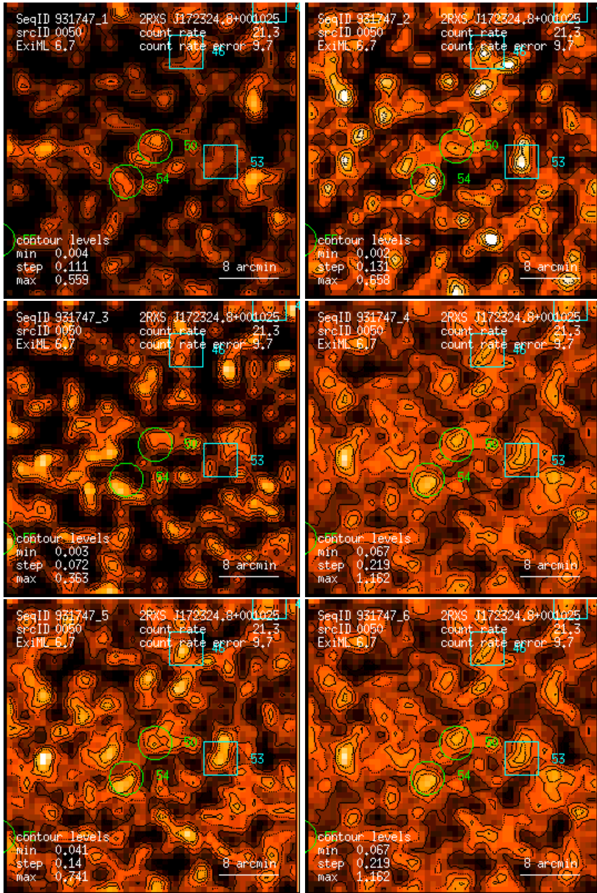
Figure 50: RASS 931747: detection 0050: band rate images, Gaussian filter: (1) PSPC channels 11 – 41, (2) 52 – 90, (3) 91 – 201, (4) 11 – 235, (5) 52 – 201, (6) 11 – 201. Broad band rates in counts/ks. Band rate contour levels in counts/ks/arcmin 2 .
