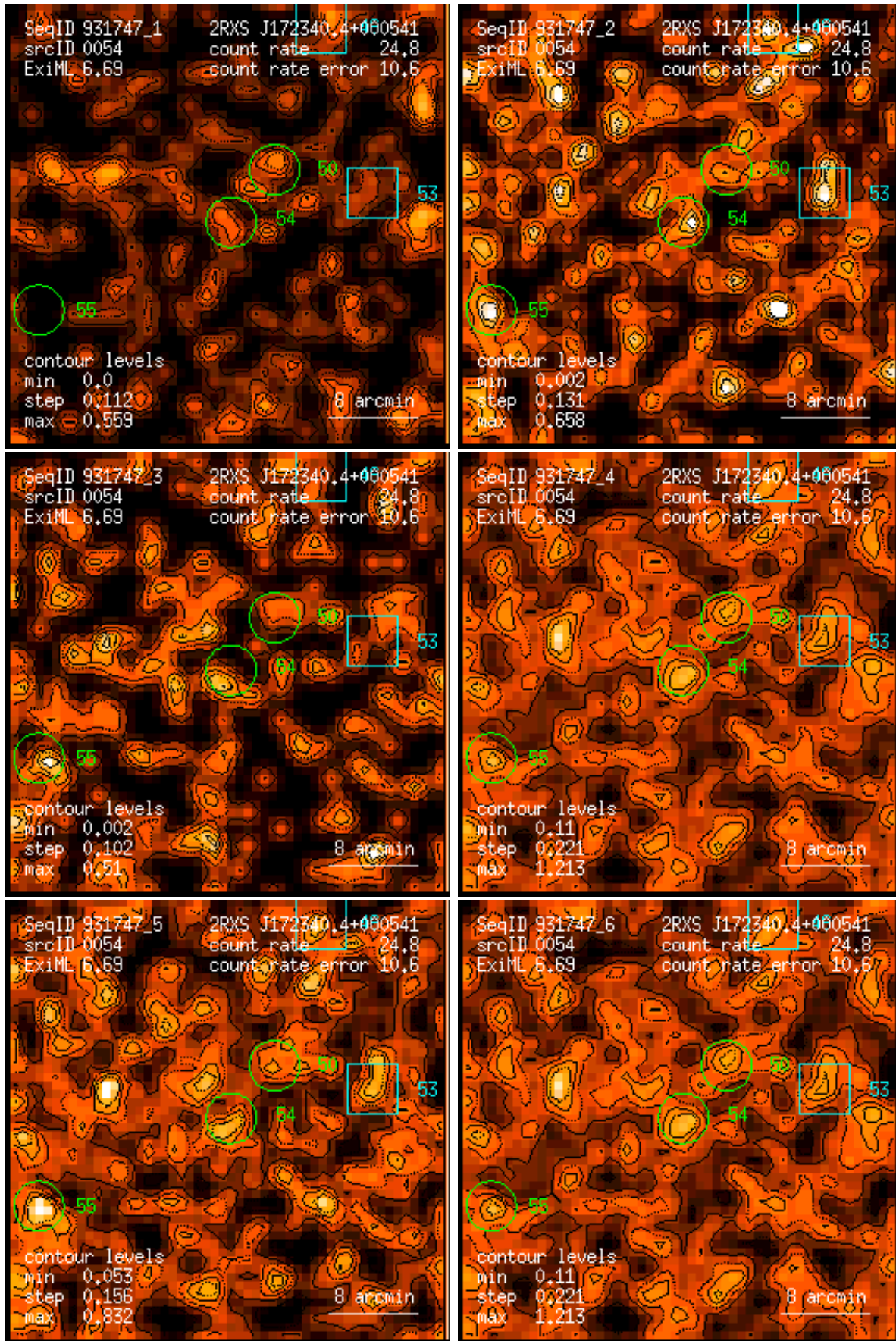
Figure 54: RASS 931747: detection 0054: band rate images, Gaussian filter: (1) PSPC channels 11 – 41, (2) 52 – 90, (3) 91 – 201, (4) 11 – 235, (5) 52 – 201, (6) 11 – 201. Broad band rates in counts/ks. Band rate contour levels in counts/ks/arcmin 2 .
