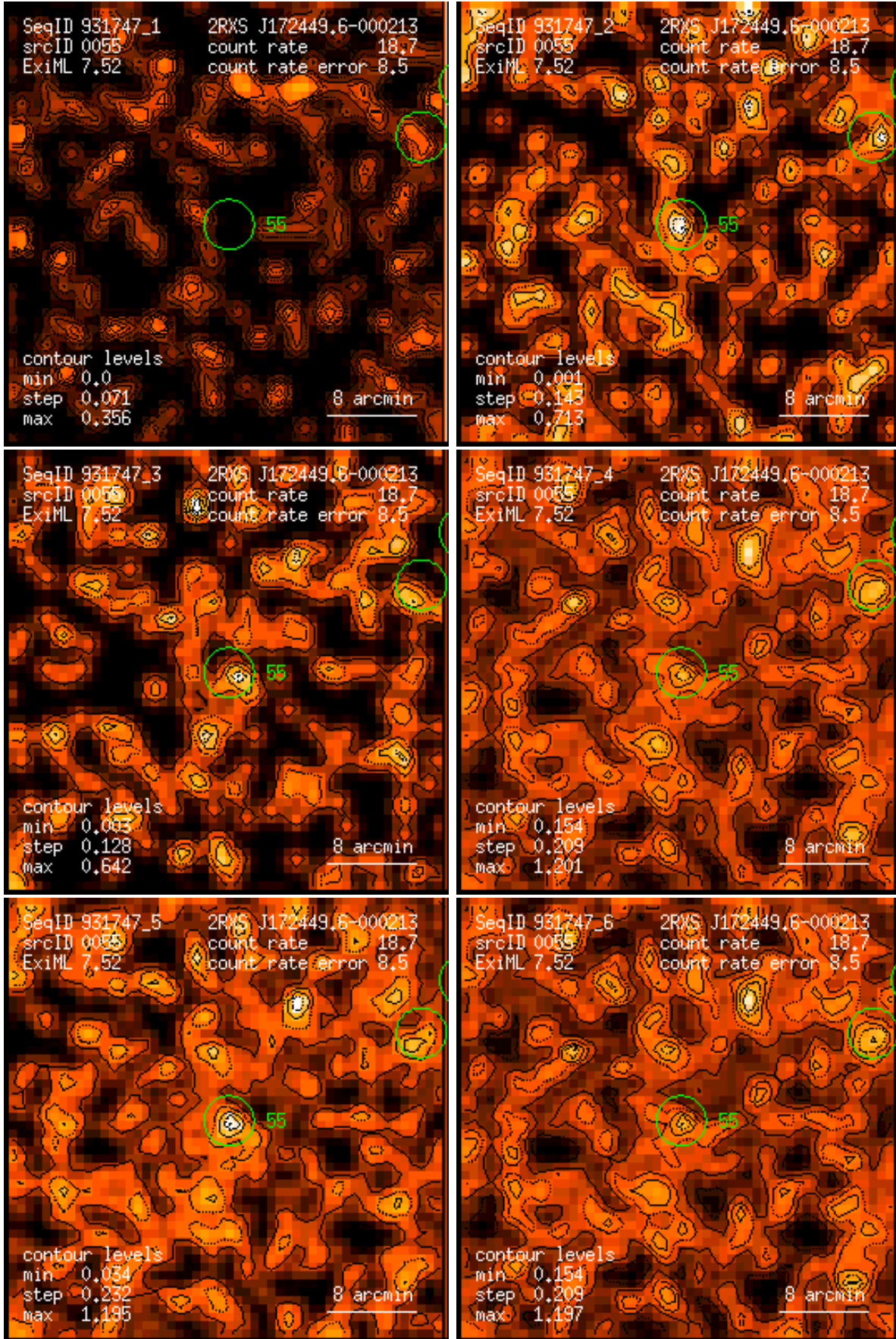
Figure 55: RASS 931747: detection 0055: band rate images, Gaussian filter: (1) PSPC channels 11 – 41, (2) 52 – 90, (3) 91 – 201, (4) 11 – 235, (5) 52 – 201, (6) 11 – 201. Broad band rates in counts/ks. Band rate contour levels in counts/ks/arcmin 2 .
