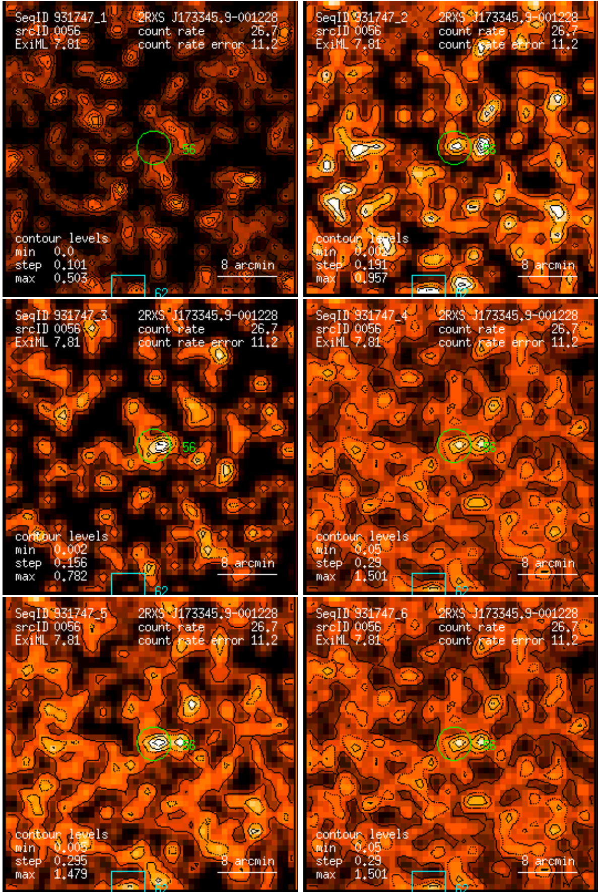
Figure 56: RASS 931747: detection 0056: band rate images, Gaussian filter: (1) PSPC channels 11 – 41, (2) 52 – 90, (3) 91 – 201, (4) 11 – 235, (5) 52 – 201, (6) 11 – 201. Broad band rates in counts/ks. Band rate contour levels in counts/ks/arcmin 2 .
