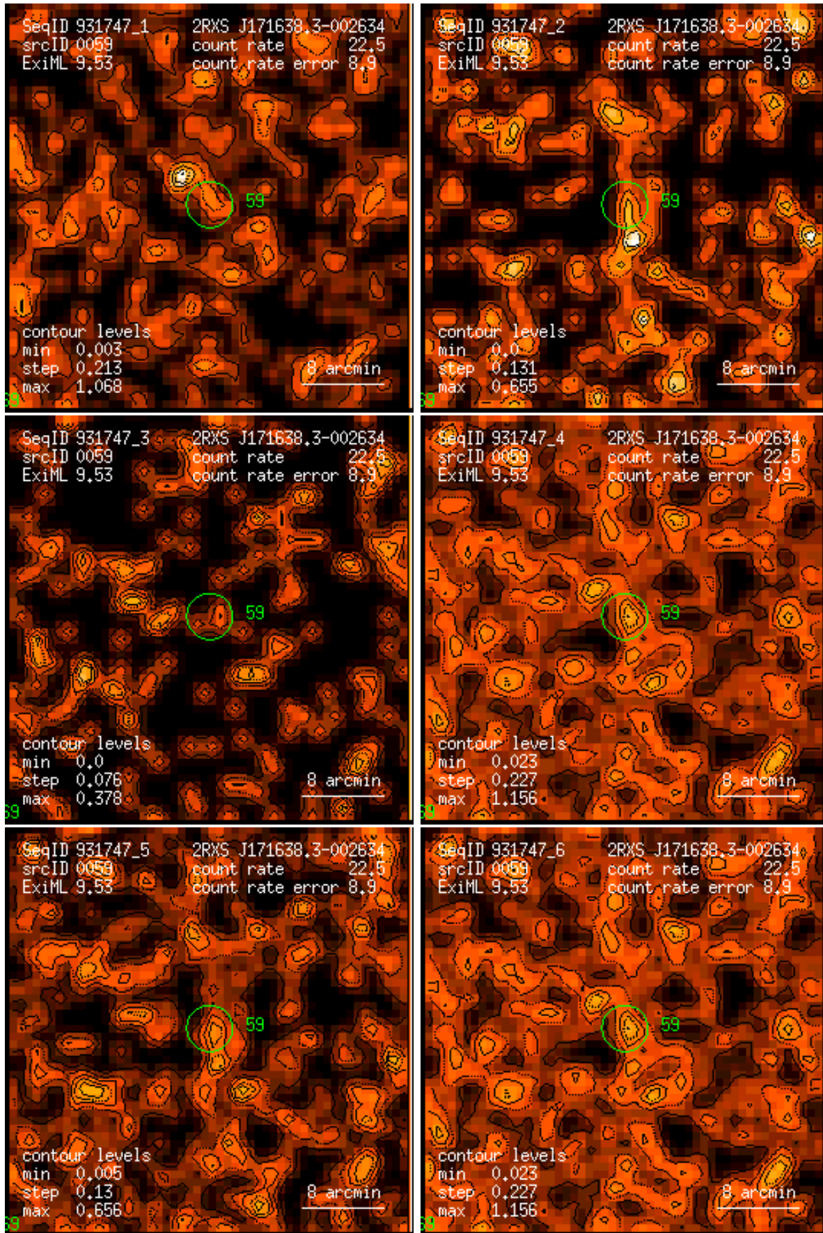
Figure 59: RASS 931747: detection 0059: band rate images, Gaussian filter: (1) PSPC channels 11 – 41, (2) 52 – 90, (3) 91 – 201, (4) 11 – 235, (5) 52 – 201, (6) 11 – 201. Broad band rates in counts/ks. Band rate contour levels in counts/ks/arcmin 2 .
