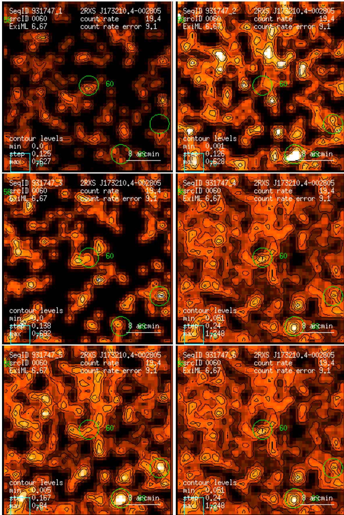
Figure 60: RASS 931747: detection 0060: band rate images, Gaussian filter: (1) PSPC channels 11 – 41, (2) 52 – 90, (3) 91 – 201, (4) 11 – 235, (5) 52 – 201, (6) 11 – 201. Broad band rates in counts/ks. Band rate contour levels in counts/ks/arcmin 2 .
