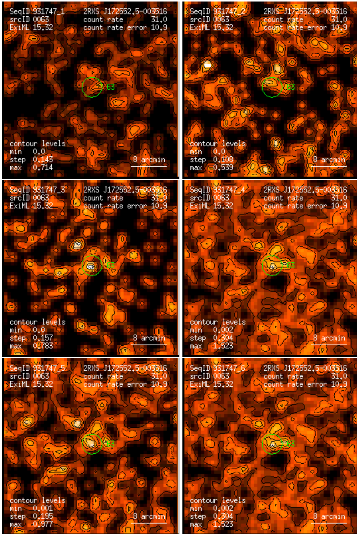
Figure 63: RASS 931747: detection 0063: band rate images, Gaussian filter: (1) PSPC channels 11 – 41, (2) 52 – 90, (3) 91 – 201, (4) 11 – 235, (5) 52 – 201, (6) 11 – 201. Broad band rates in counts/ks. Band rate contour levels in counts/ks/arcmin 2 .
