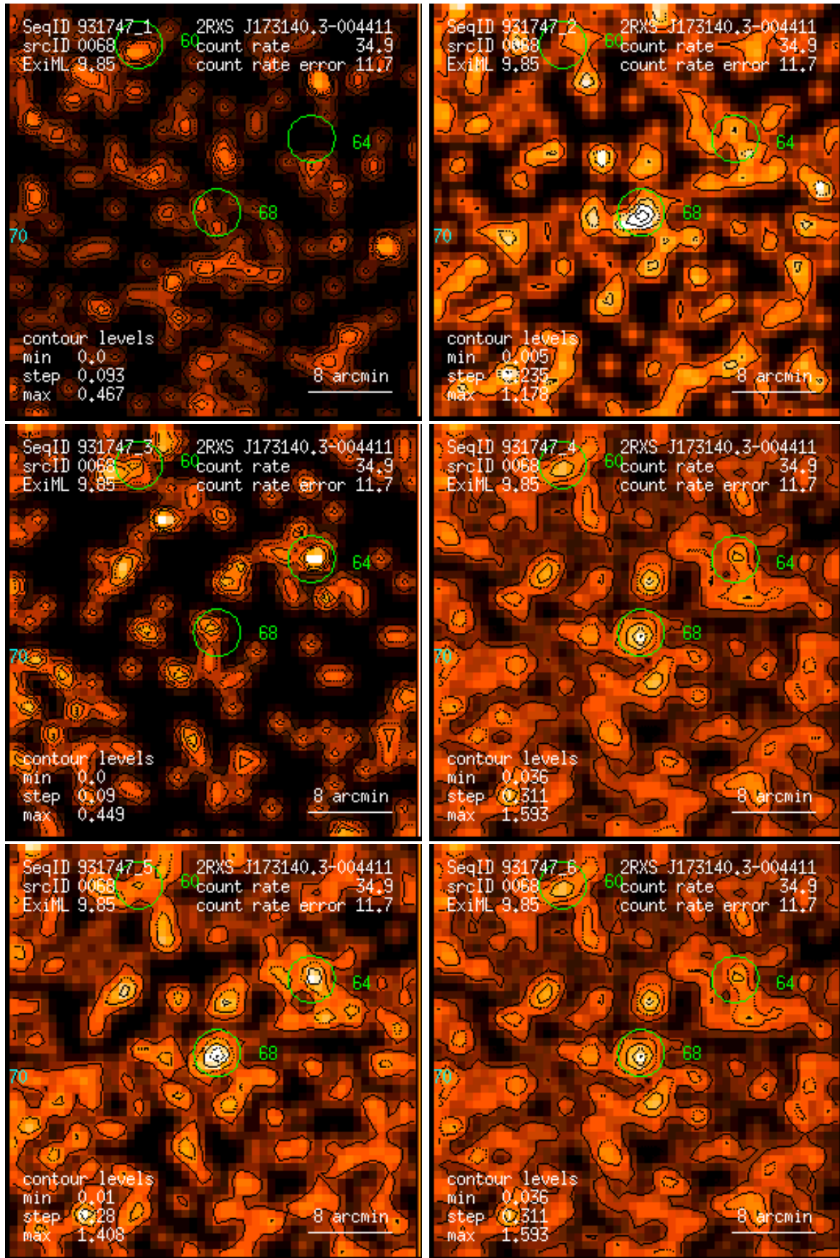
Figure 68: RASS 931747: detection 0068: band rate images, Gaussian filter: (1) PSPC channels 11 – 41, (2) 52 – 90, (3) 91 – 201, (4) 11 – 235, (5) 52 – 201, (6) 11 – 201. Broad band rates in counts/ks. Band rate contour levels in counts/ks/arcmin 2 .
