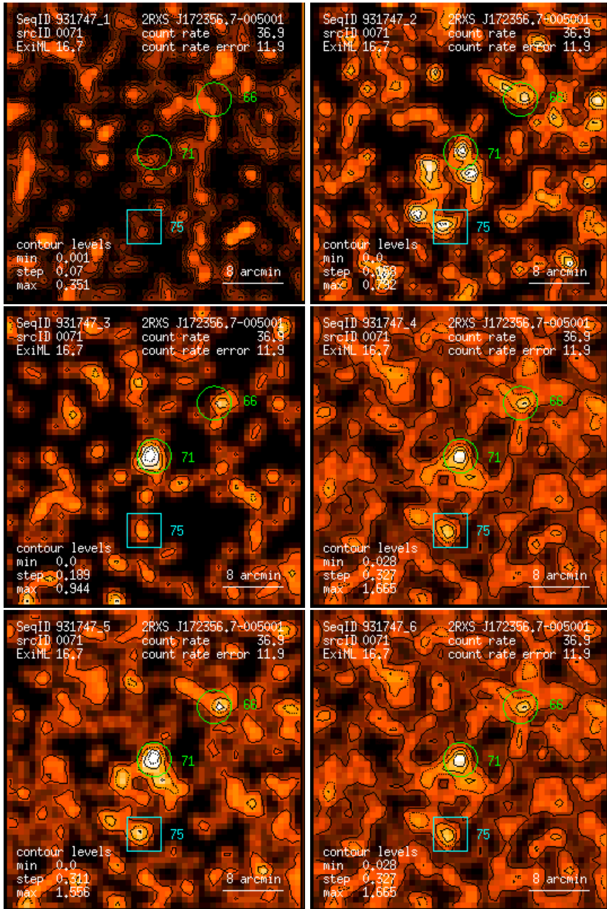
Figure 71: RASS 931747: detection 0071: band rate images, Gaussian filter: (1) PSPC channels 11 – 41, (2) 52 – 90, (3) 91 – 201, (4) 11 – 235, (5) 52 – 201, (6) 11 – 201. Broad band rates in counts/ks. Band rate contour levels in counts/ks/arcmin 2 .
