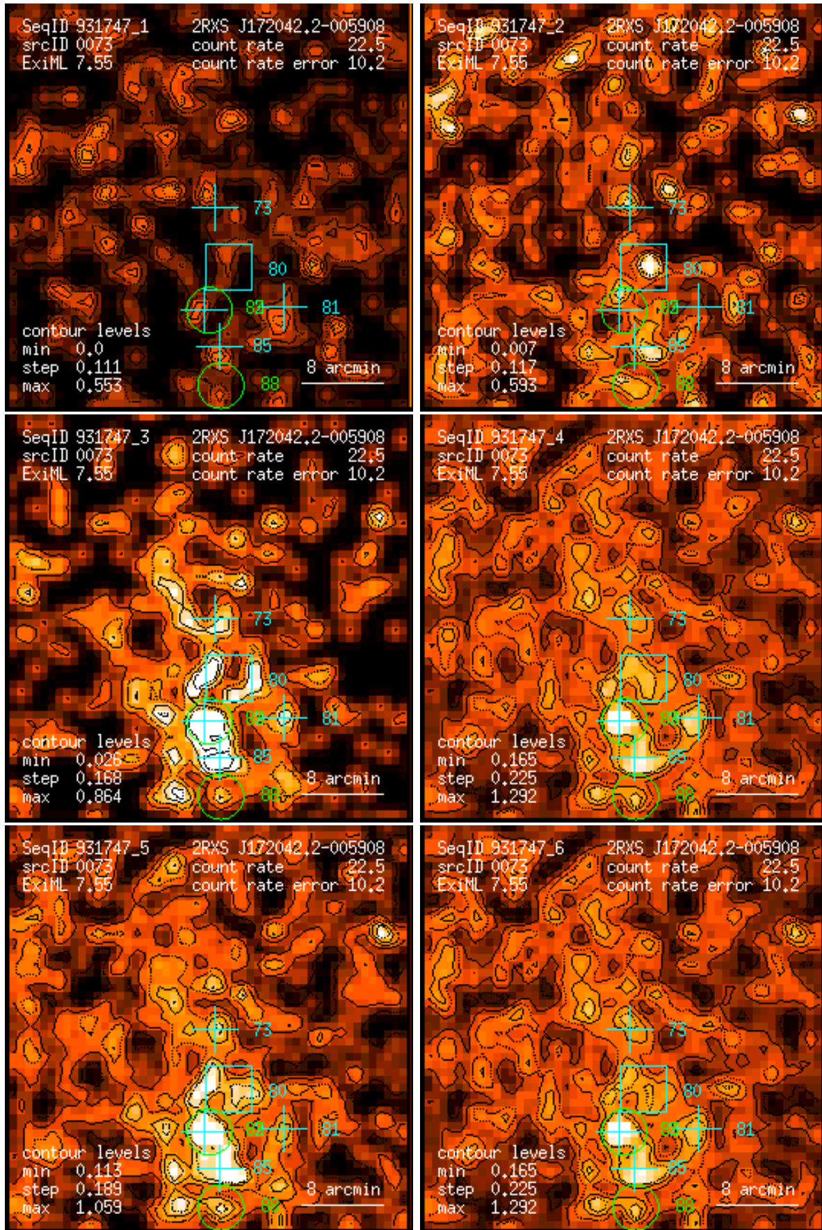
Figure 73: RASS 931747: detection 0073: band rate images, Gaussian filter: (1) PSPC channels 11 – 41, (2) 52 – 90, (3) 91 – 201, (4) 11 – 235, (5) 52 – 201, (6) 11 – 201. Broad band rates in counts/ks. Band rate contour levels in counts/ks/arcmin 2 .
