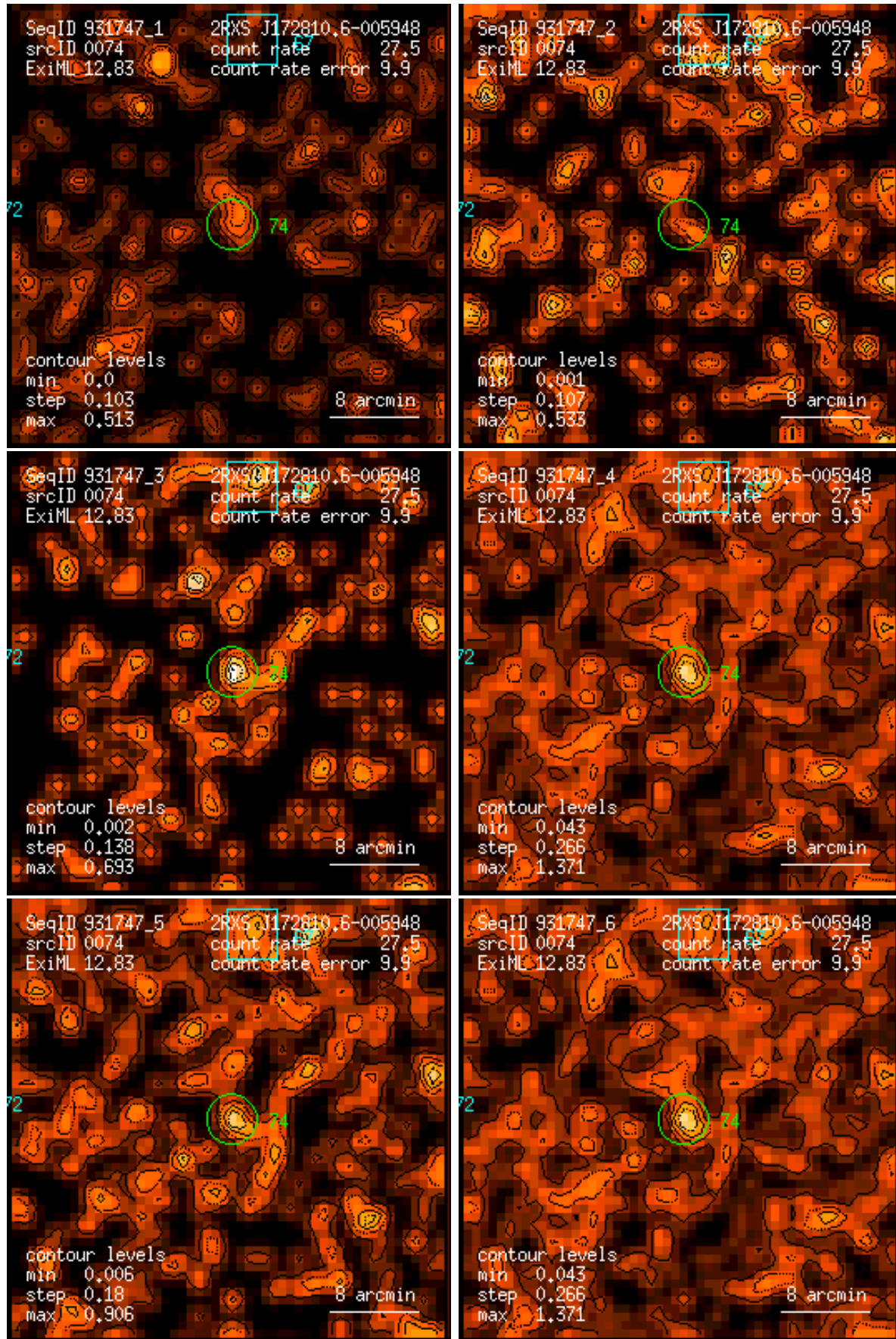
Figure 74: RASS 931747: detection 0074: band rate images, Gaussian filter: (1) PSPC channels 11 – 41, (2) 52 – 90, (3) 91 – 201, (4) 11 – 235, (5) 52 – 201, (6) 11 – 201. Broad band rates in counts/ks. Band rate contour levels in counts/ks/arcmin 2 .
