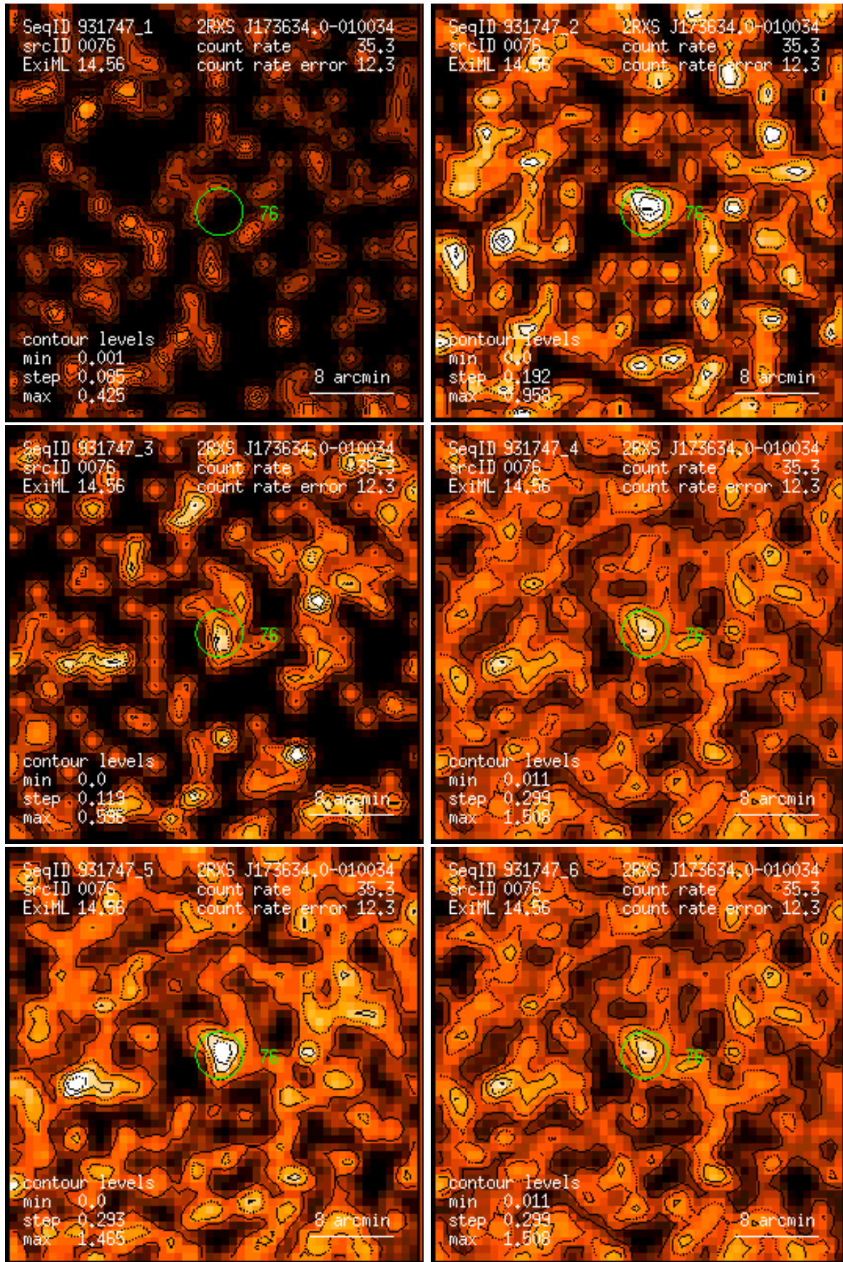
Figure 76: RASS 931747: detection 0076: band rate images, Gaussian filter: (1) PSPC channels 11 – 41, (2) 52 – 90, (3) 91 – 201, (4) 11 – 235, (5) 52 – 201, (6) 11 – 201. Broad band rates in counts/ks. Band rate contour levels in counts/ks/arcmin 2 .
